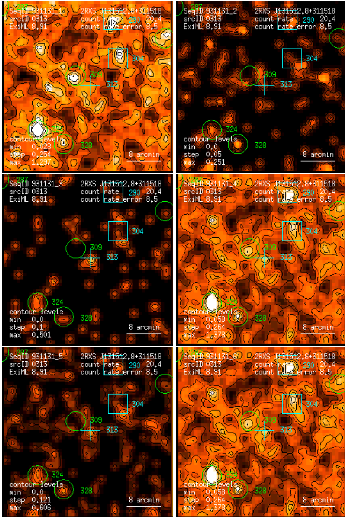
Figure 313: RASS 931131: detection 0313: band rate images, Gaussian filter: (1) PSPC channels 11 – 41, (2) 52 – 90, (3) 91 – 201, (4) 11 – 235, (5) 52 – 201, (6) 11 – 201. Broad band rates in counts/ks. Band rate contour levels in counts/ks/arcmin 2 .
