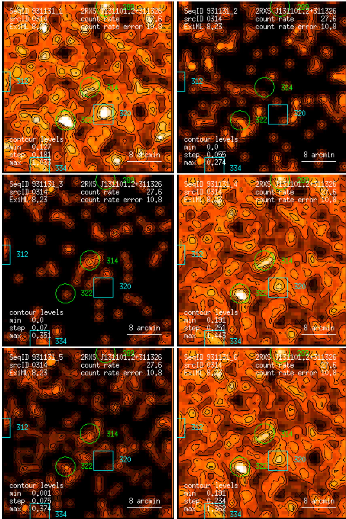
Figure 314: RASS 931131: detection 0314: band rate images, Gaussian filter: (1) PSPC channels 11 – 41, (2) 52 – 90, (3) 91 – 201, (4) 11 – 235, (5) 52 – 201, (6) 11 – 201. Broad band rates in counts/ks. Band rate contour levels in counts/ks/arcmin 2 .
