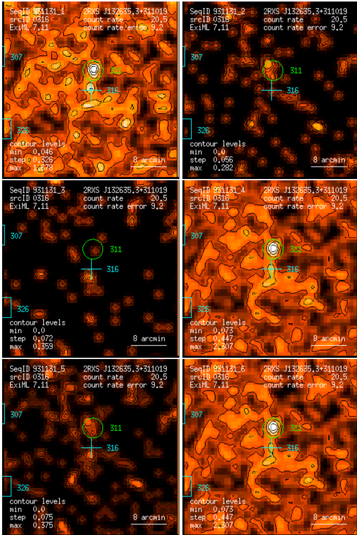
Figure 316: RASS 931131: detection 0316: band rate images, Gaussian filter: (1) PSPC channels 11 – 41, (2) 52 – 90, (3) 91 – 201, (4) 11 – 235, (5) 52 – 201, (6) 11 – 201. Broad band rates in counts/ks. Band rate contour levels in counts/ks/arcmin 2 .
