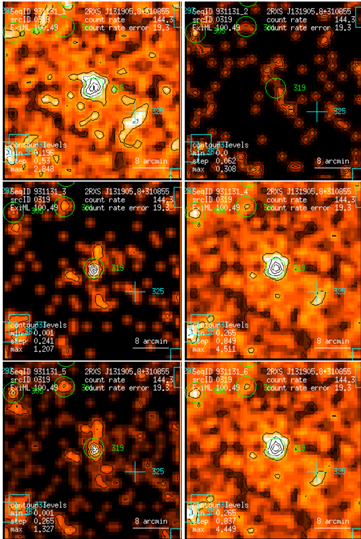
Figure 319: RASS 931131: detection 0319: band rate images, Gaussian filter: (1) PSPC channels 11 – 41, (2) 52 – 90, (3) 91 – 201, (4) 11 – 235, (5) 52 – 201, (6) 11 – 201. Broad band rates in counts/ks. Band rate contour levels in counts/ks/arcmin 2 .
