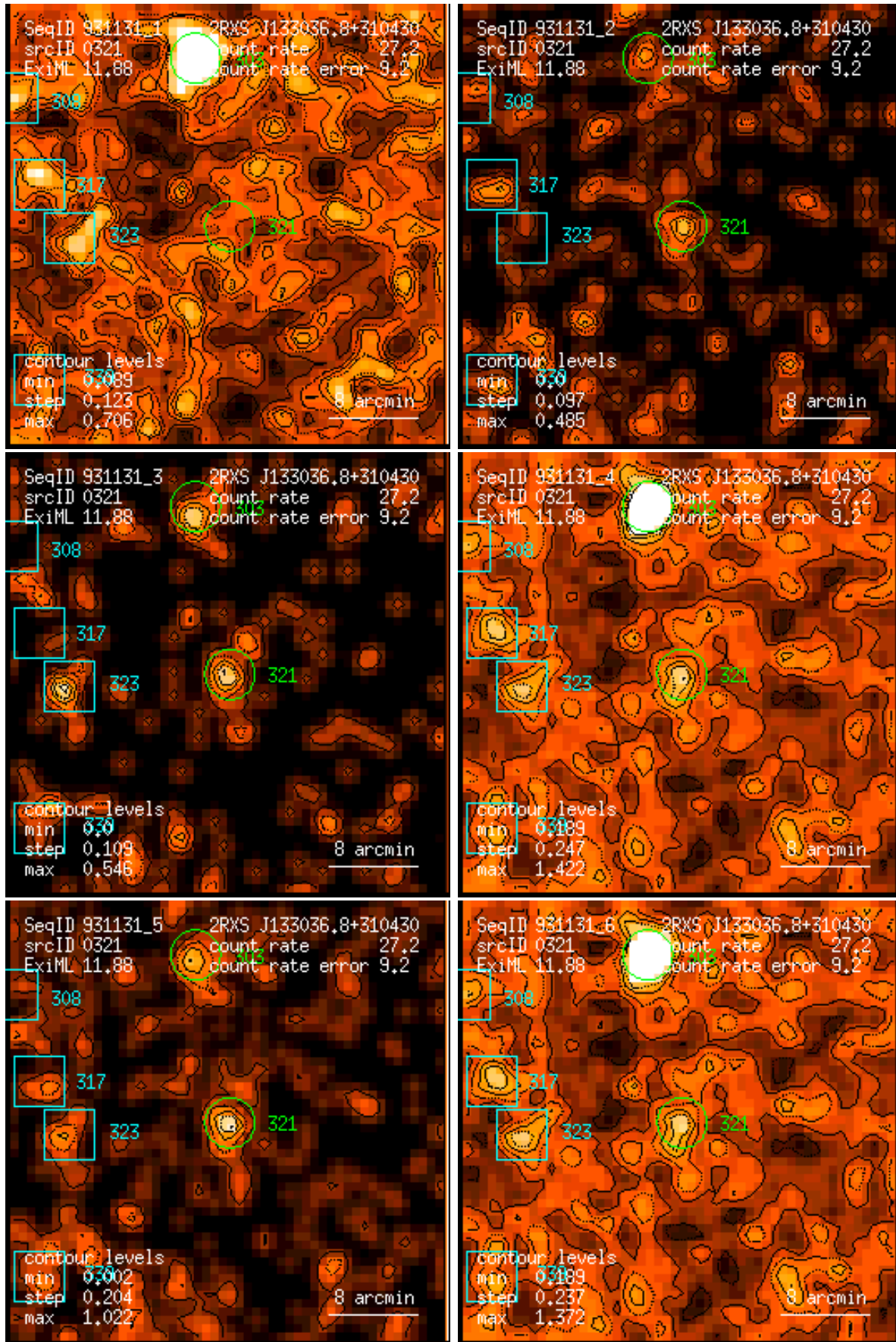
Figure 321: RASS 931131: detection 0321: band rate images, Gaussian filter: (1) PSPC channels 11 – 41, (2) 52 – 90, (3) 91 – 201, (4) 11 – 235, (5) 52 – 201, (6) 11 – 201. Broad band rates in counts/ks. Band rate contour levels in counts/ks/arcmin 2 .
