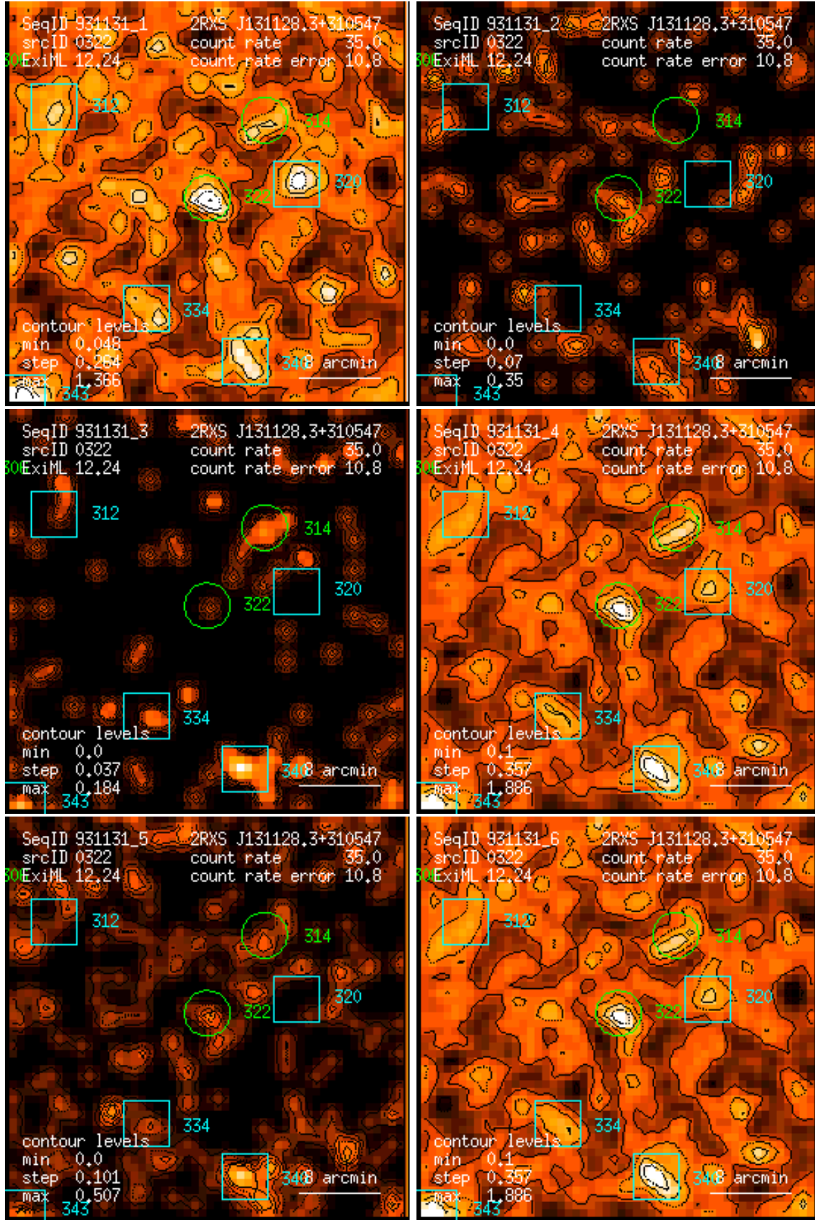
Figure 322: RASS 931131: detection 0322: band rate images, Gaussian filter: (1) PSPC channels 11 – 41, (2) 52 – 90, (3) 91 – 201, (4) 11 – 235, (5) 52 – 201, (6) 11 – 201. Broad band rates in counts/ks. Band rate contour levels in counts/ks/arcmin 2 .
