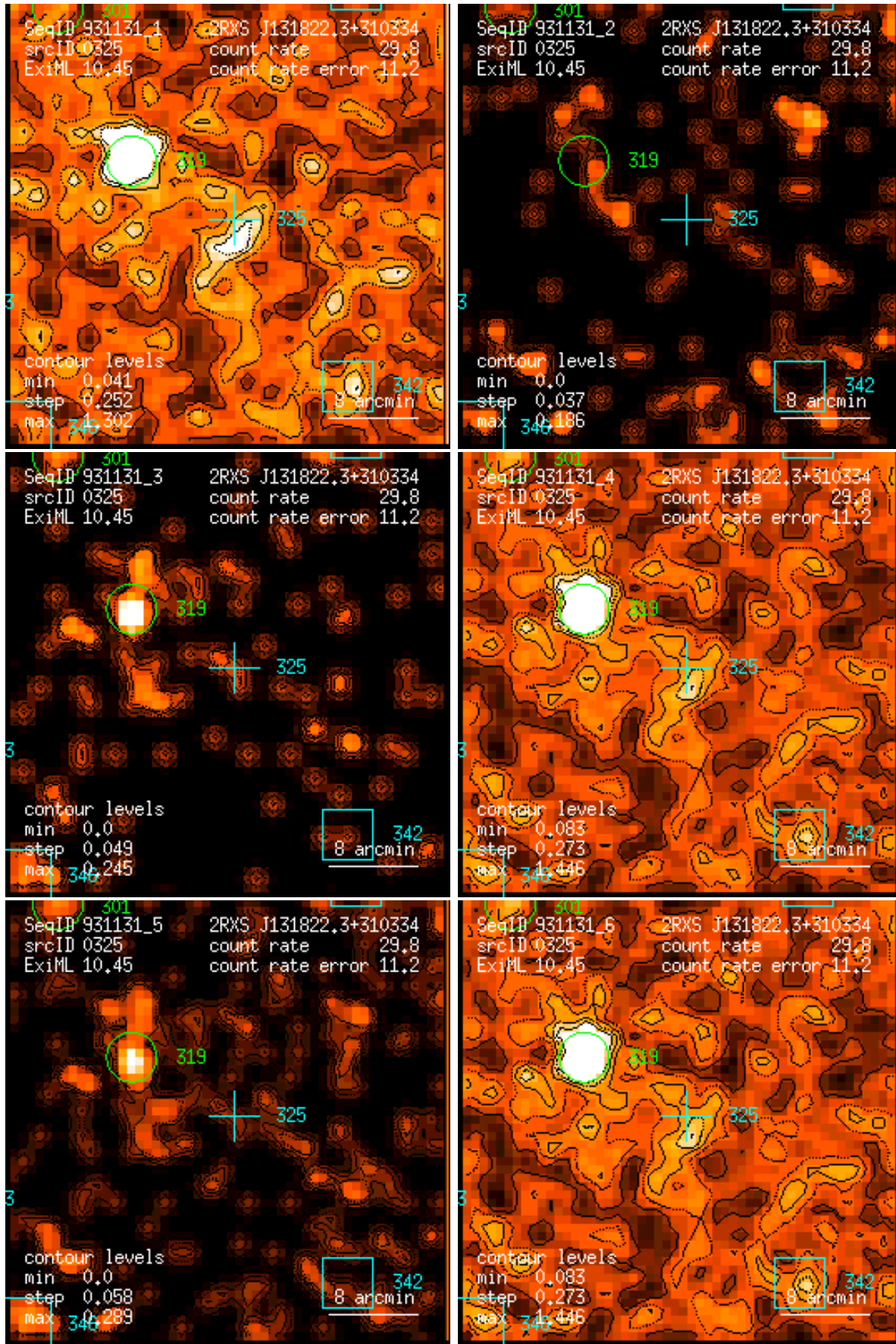
Figure 325: RASS 931131: detection 0325: band rate images, Gaussian filter: (1) PSPC channels 11 – 41, (2) 52 – 90, (3) 91 – 201, (4) 11 – 235, (5) 52 – 201, (6) 11 – 201. Broad band rates in counts/ks. Band rate contour levels in counts/ks/arcmin 2 .
