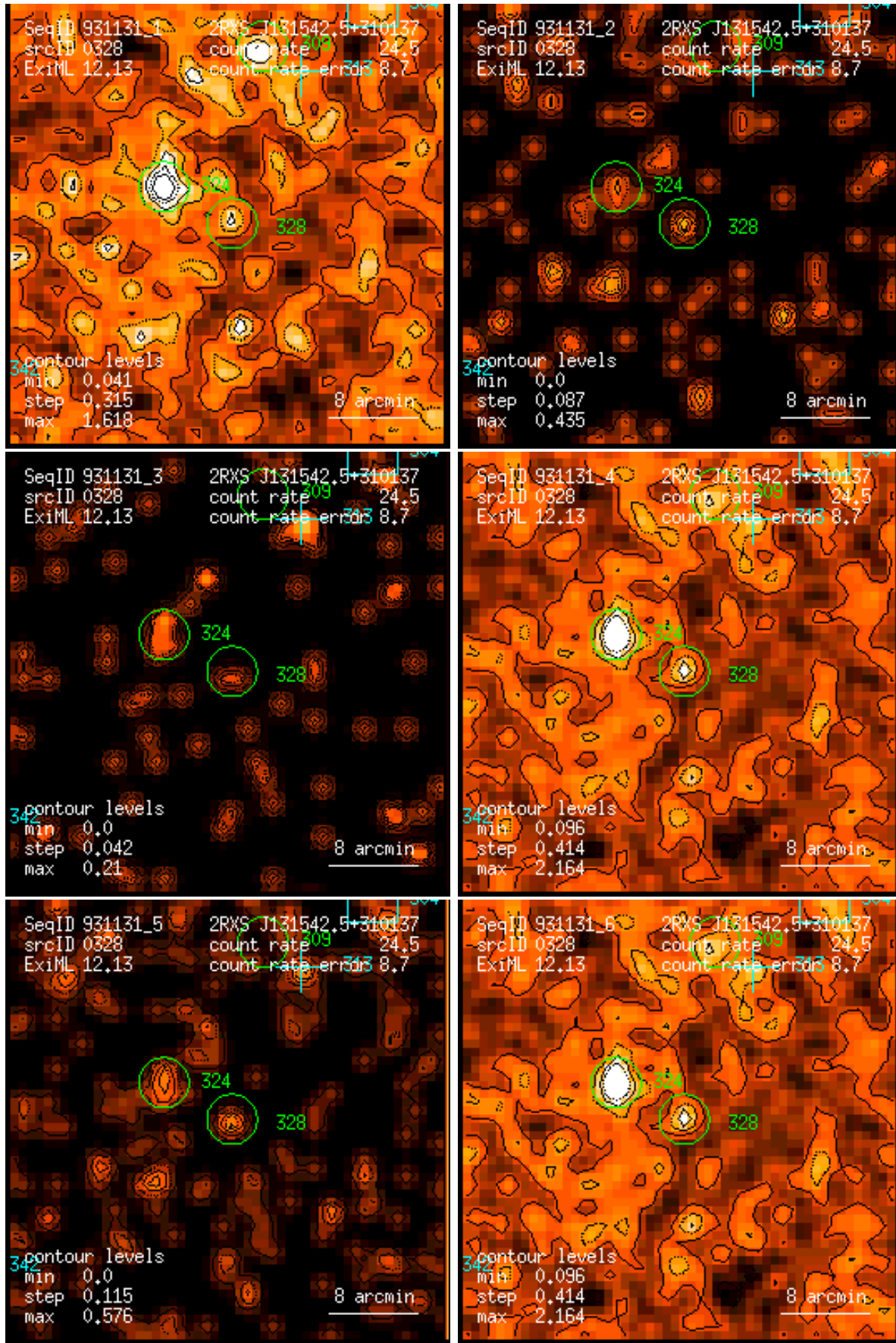
Figure 328: RASS 931131: detection 0328: band rate images, Gaussian filter: (1) PSPC channels 11 – 41, (2) 52 – 90, (3) 91 – 201, (4) 11 – 235, (5) 52 – 201, (6) 11 – 201. Broad band rates in counts/ks. Band rate contour levels in counts/ks/arcmin 2 .
