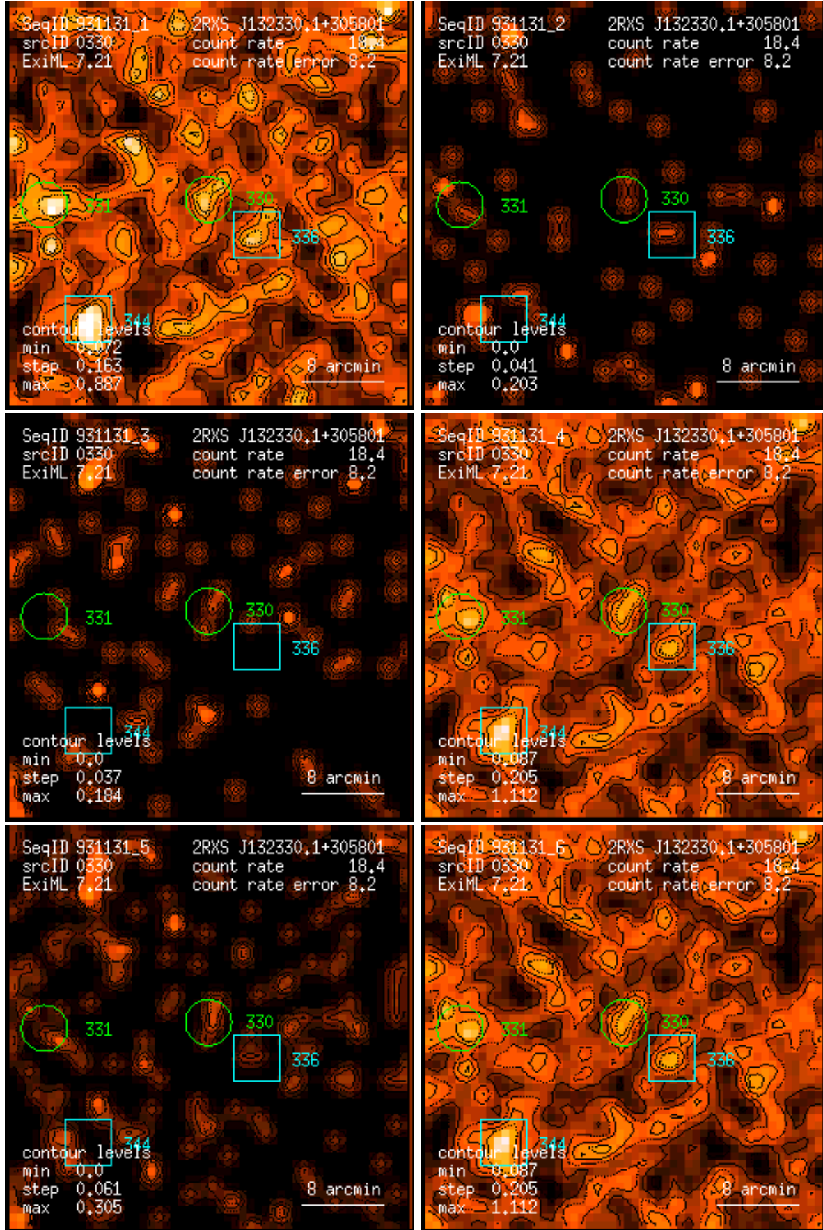
Figure 330: RASS 931131: detection 0330: band rate images, Gaussian filter: (1) PSPC channels 11 – 41, (2) 52 – 90, (3) 91 – 201, (4) 11 – 235, (5) 52 – 201, (6) 11 – 201. Broad band rates in counts/ks. Band rate contour levels in counts/ks/arcmin 2 .
