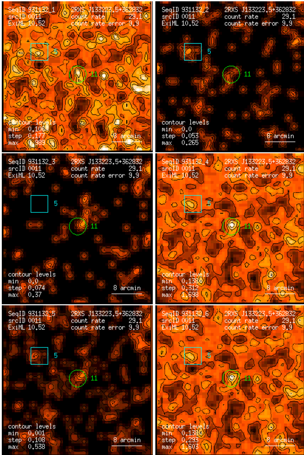
Figure 11: RASS 931132: detection 0011: band rate images, Gaussian filter: (1) PSPC channels 11 – 41, (2) 52 – 90, (3) 91 – 201, (4) 11 – 235, (5) 52 – 201, (6) 11 – 201. Broad band rates in counts/ks. Band rate contour levels in counts/ks/arcmin 2 .
