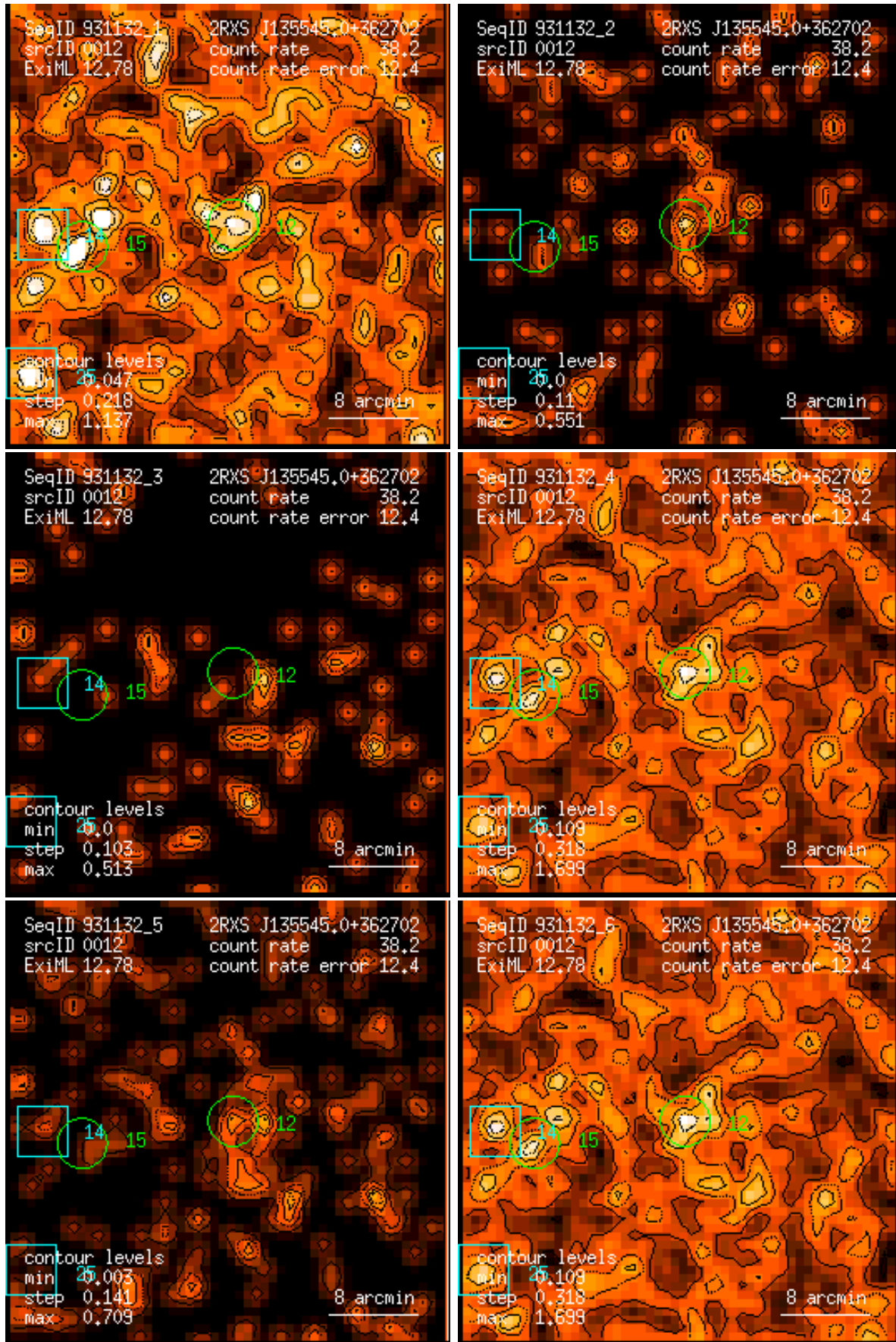
Figure 12: RASS 931132: detection 0012: band rate images, Gaussian filter: (1) PSPC channels 11 – 41, (2) 52 – 90, (3) 91 – 201, (4) 11 – 235, (5) 52 – 201, (6) 11 – 201. Broad band rates in counts/ks. Band rate contour levels in counts/ks/arcmin 2 .
