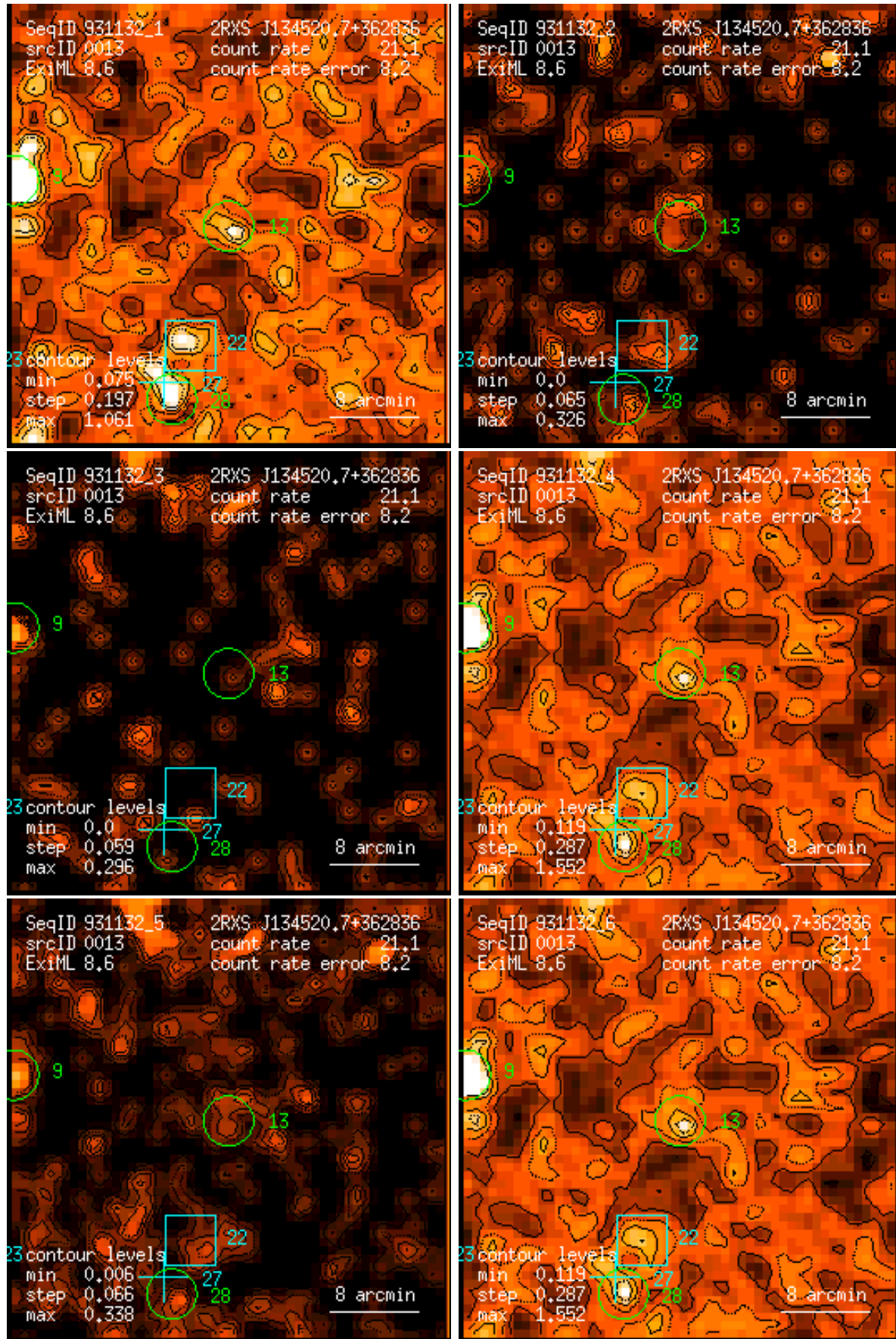
Figure 13: RASS 931132: detection 0013: band rate images, Gaussian filter: (1) PSPC channels 11 – 41, (2) 52 – 90, (3) 91 – 201, (4) 11 – 235, (5) 52 – 201, (6) 11 – 201. Broad band rates in counts/ks. Band rate contour levels in counts/ks/arcmin 2 .
