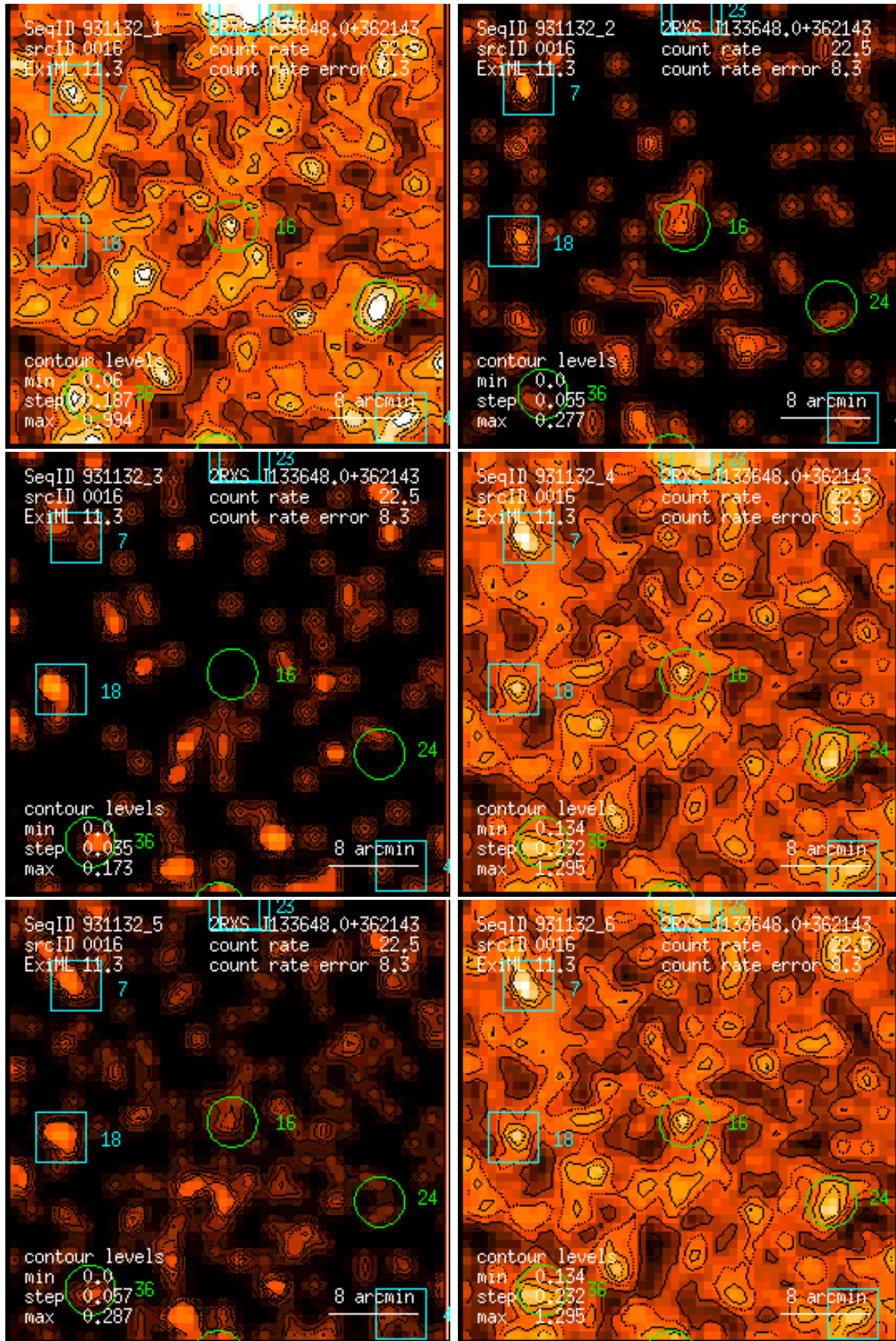
Figure 16: RASS 931132: detection 0016: band rate images, Gaussian filter: (1) PSPC channels 11 – 41, (2) 52 – 90, (3) 91 – 201, (4) 11 – 235, (5) 52 – 201, (6) 11 – 201. Broad band rates in counts/ks. Band rate contour levels in counts/ks/arcmin 2 .
