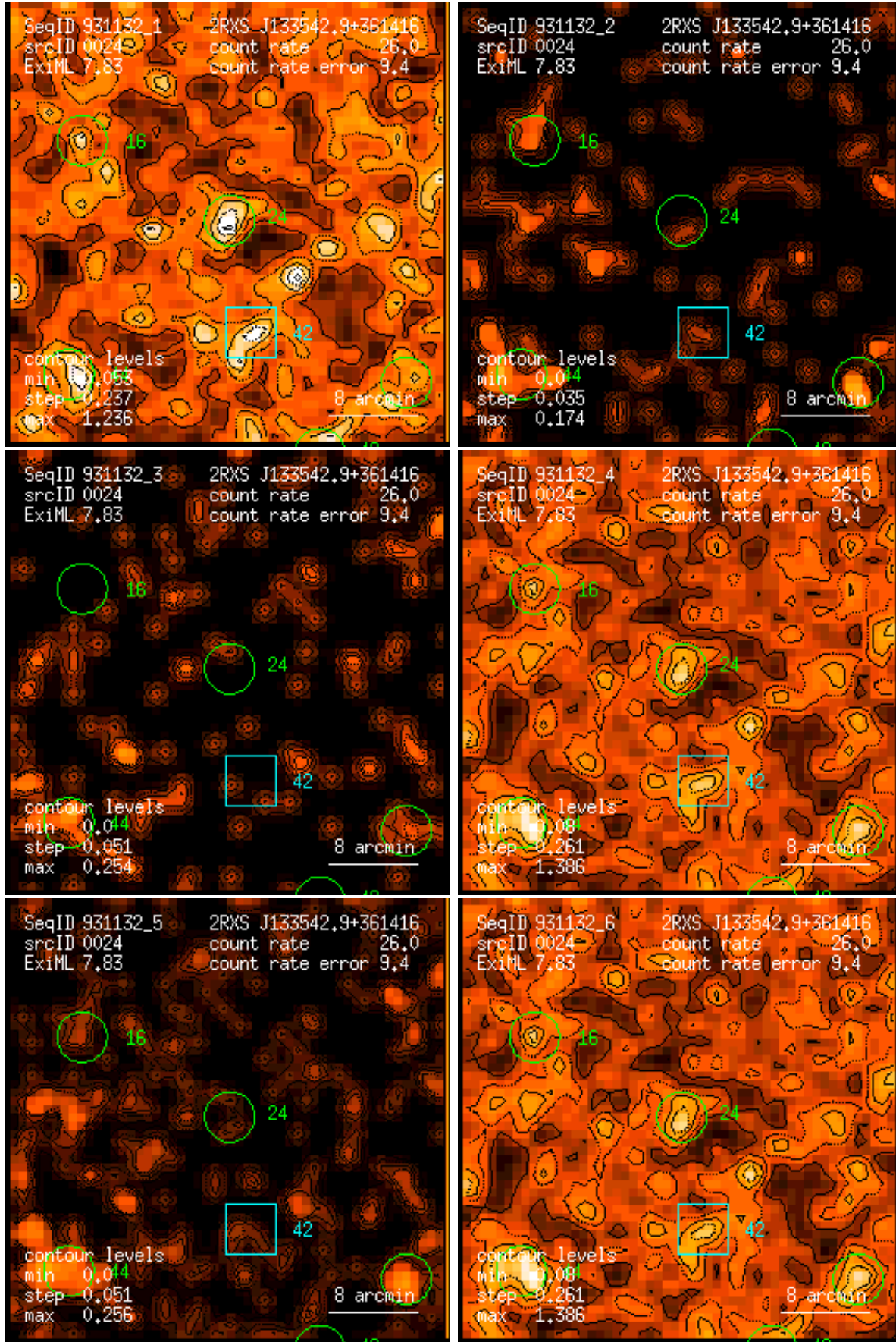
Figure 24: RASS 931132: detection 0024: band rate images, Gaussian filter: (1) PSPC channels 11 – 41, (2) 52 – 90, (3) 91 – 201, (4) 11 – 235, (5) 52 – 201, (6) 11 – 201. Broad band rates in counts/ks. Band rate contour levels in counts/ks/arcmin 2 .
