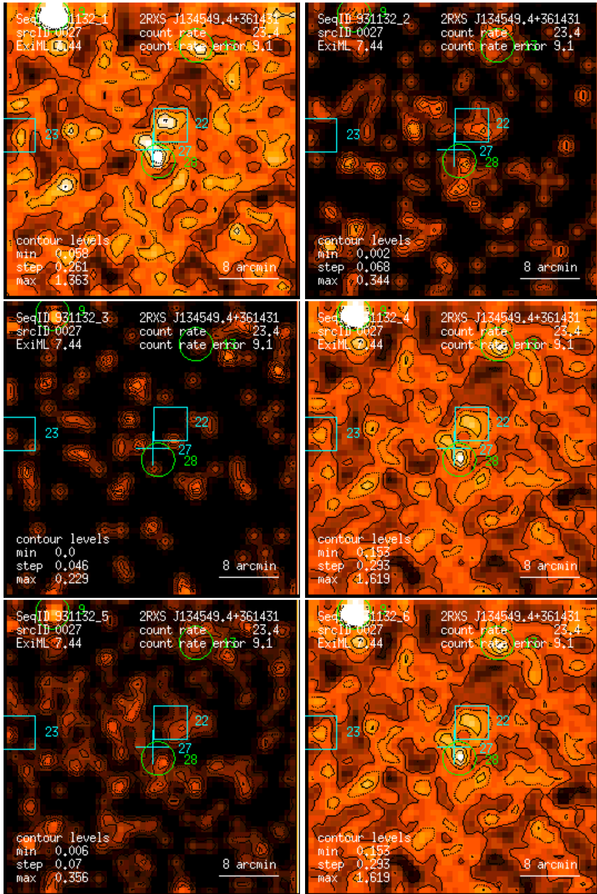
Figure 27: RASS 931132: detection 0027: band rate images, Gaussian filter: (1) PSPC channels 11 – 41, (2) 52 – 90, (3) 91 – 201, (4) 11 – 235, (5) 52 – 201, (6) 11 – 201. Broad band rates in counts/ks. Band rate contour levels in counts/ks/arcmin 2 .
