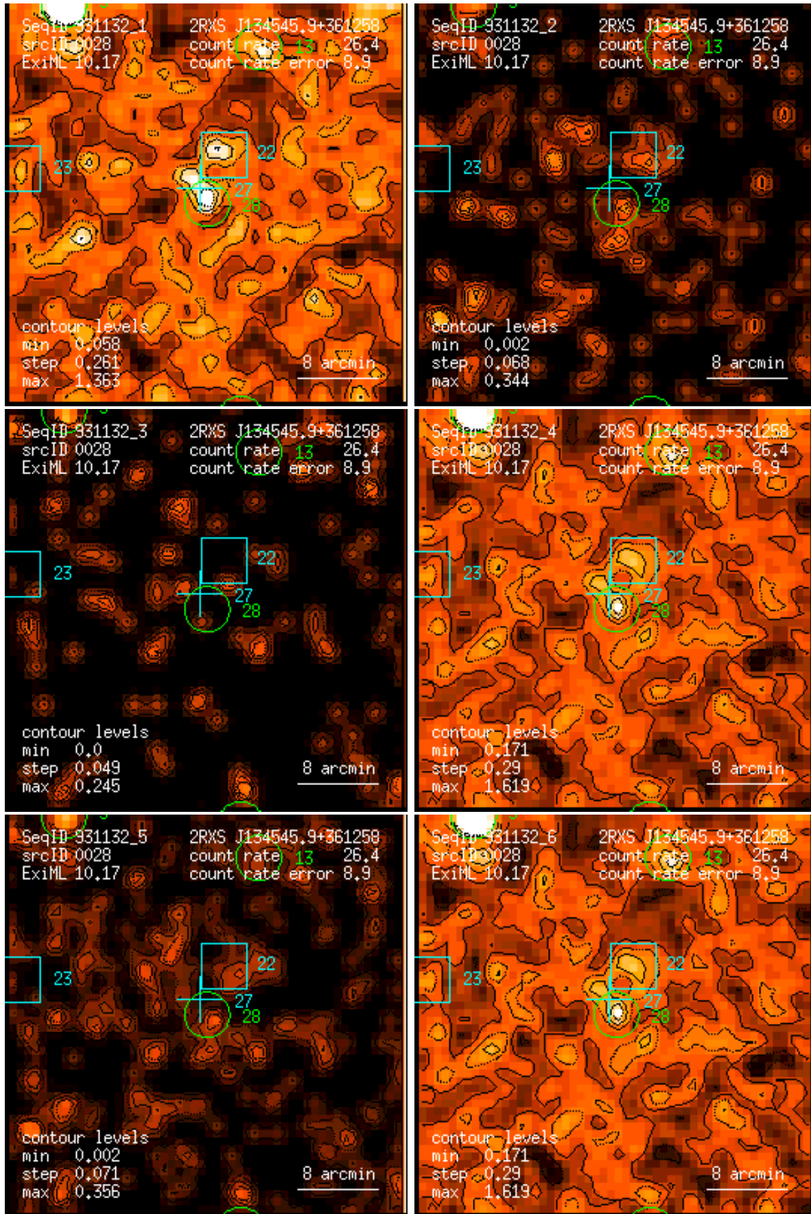
Figure 28: RASS 931132: detection 0028: band rate images, Gaussian filter: (1) PSPC channels 11 – 41, (2) 52 – 90, (3) 91 – 201, (4) 11 – 235, (5) 52 – 201, (6) 11 – 201. Broad band rates in counts/ks. Band rate contour levels in counts/ks/arcmin 2 .
