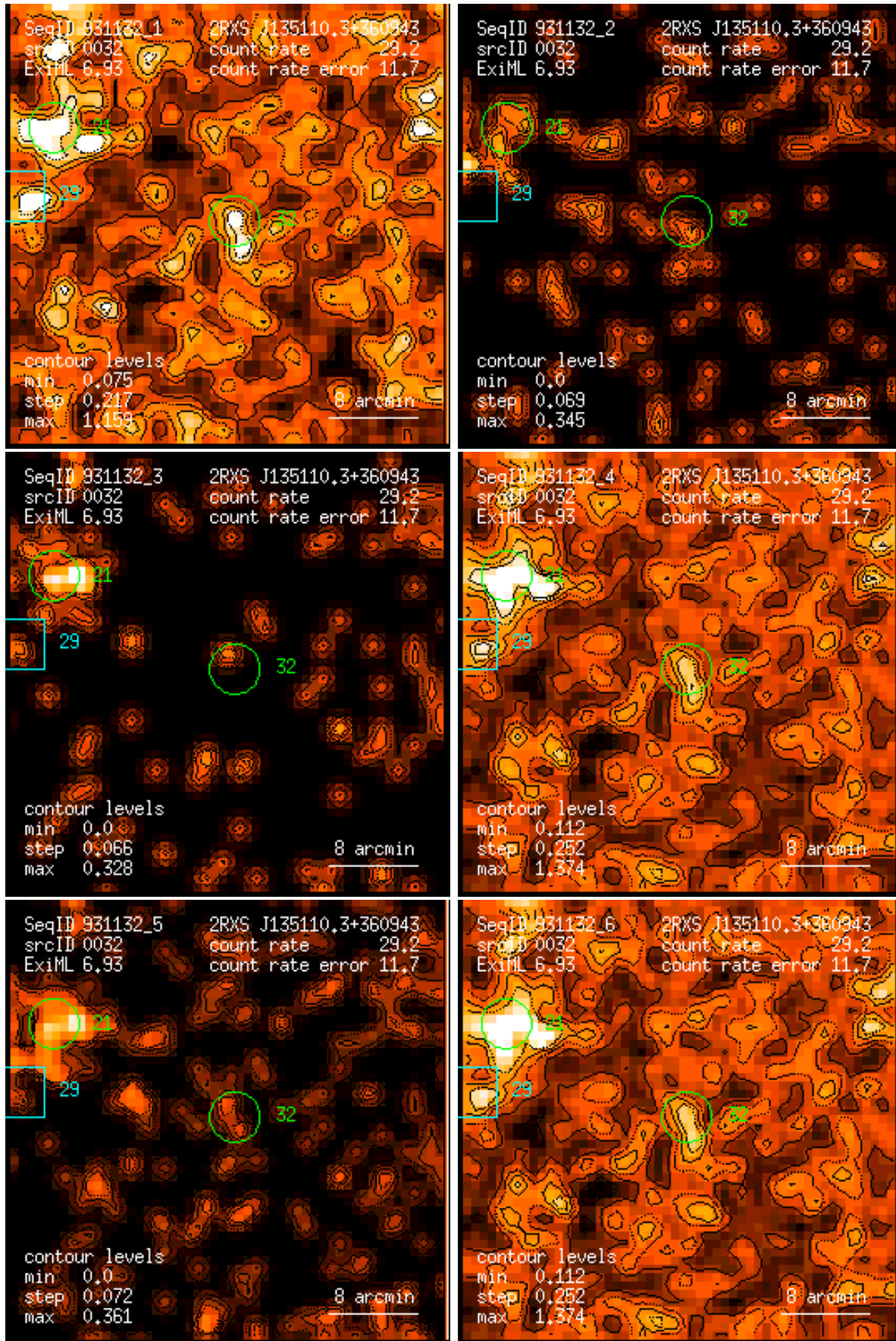
Figure 32: RASS 931132: detection 0032: band rate images, Gaussian filter: (1) PSPC channels 11 – 41, (2) 52 – 90, (3) 91 – 201, (4) 11 – 235, (5) 52 – 201, (6) 11 – 201. Broad band rates in counts/ks. Band rate contour levels in counts/ks/arcmin 2 .
