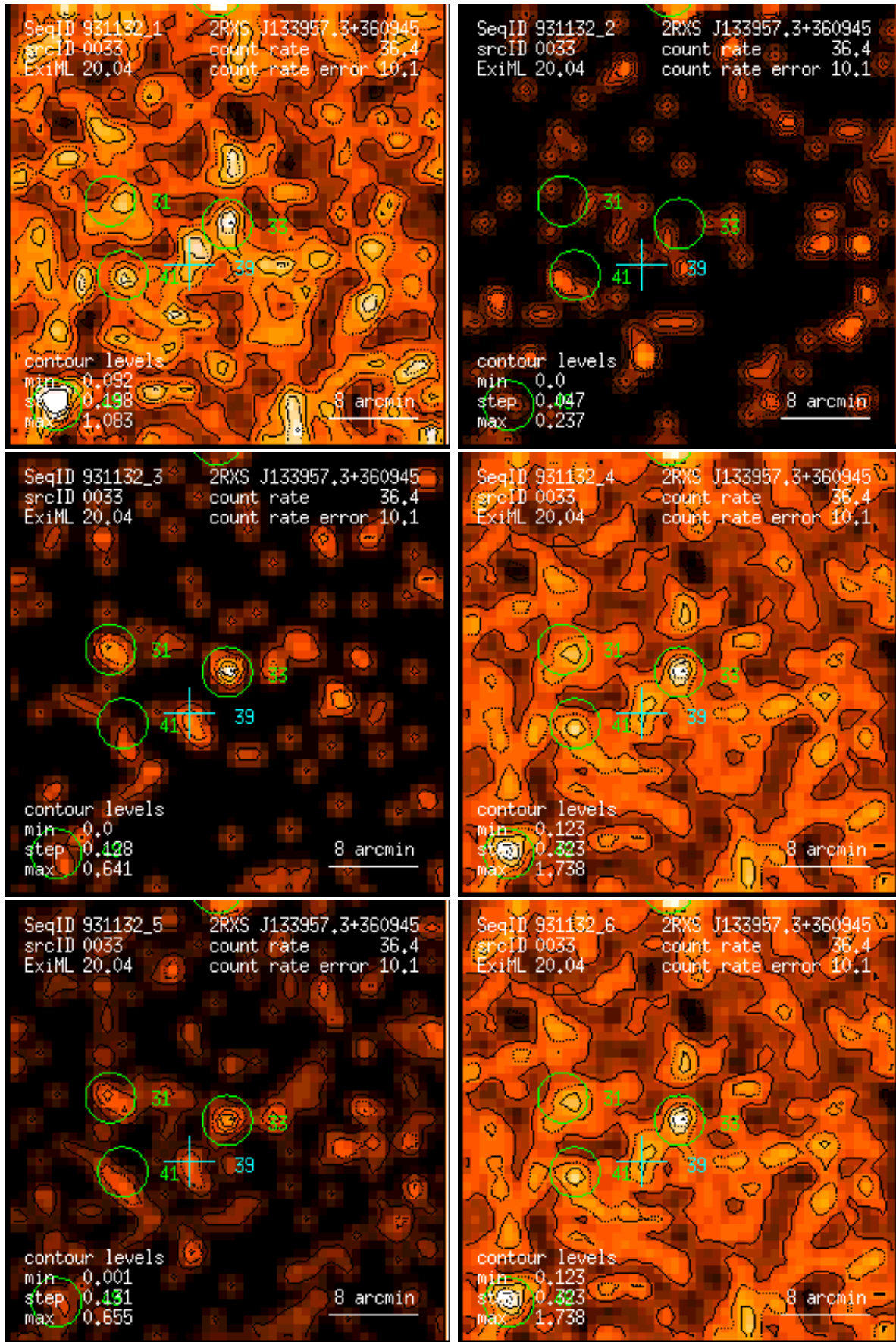
Figure 33: RASS 931132: detection 0033: band rate images, Gaussian filter: (1) PSPC channels 11 – 41, (2) 52 – 90, (3) 91 – 201, (4) 11 – 235, (5) 52 – 201, (6) 11 – 201. Broad band rates in counts/ks. Band rate contour levels in counts/ks/arcmin 2 .
