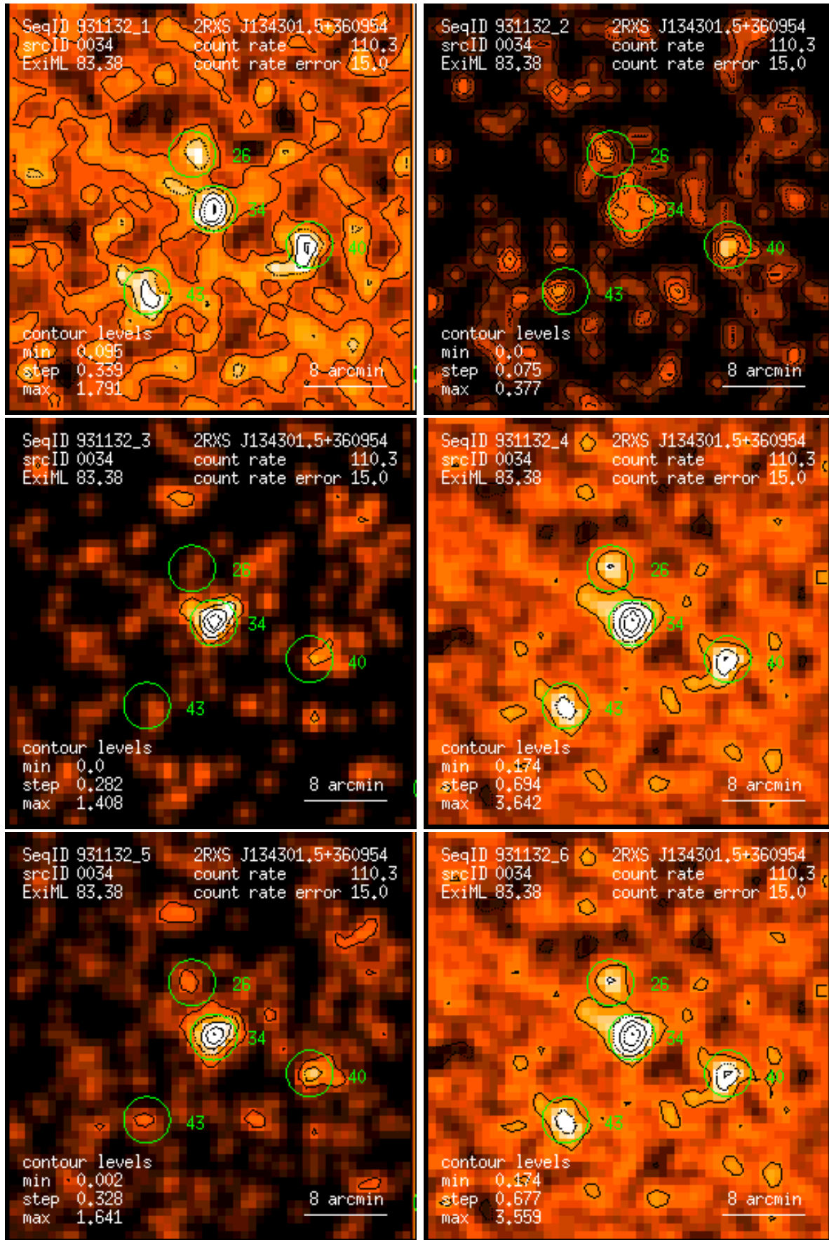
Figure 34: RASS 931132: detection 0034: band rate images, Gaussian filter: (1) PSPC channels 11 – 41, (2) 52 – 90, (3) 91 – 201, (4) 11 – 235, (5) 52 – 201, (6) 11 – 201. Broad band rates in counts/ks. Band rate contour levels in counts/ks/arcmin 2 .
