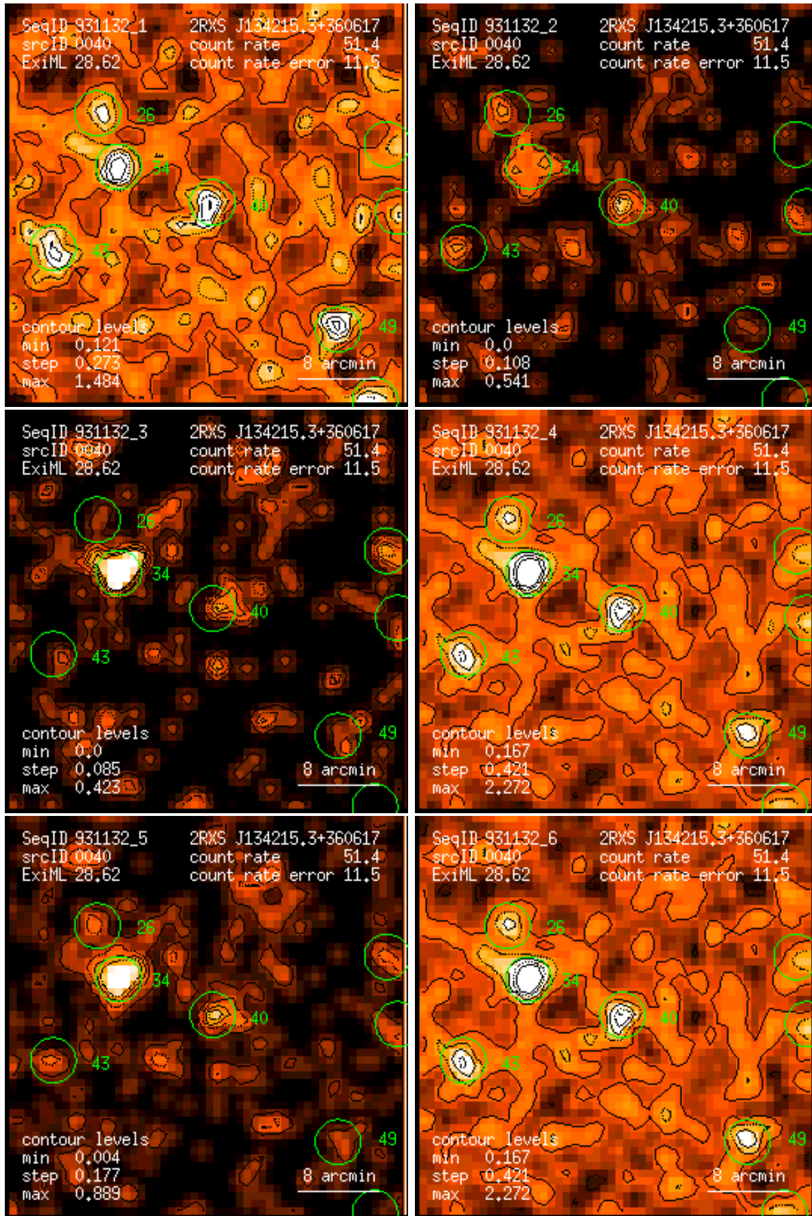
Figure 40: RASS 931132: detection 0040: band rate images, Gaussian filter: (1) PSPC channels 11 – 41, (2) 52 – 90, (3) 91 – 201, (4) 11 – 235, (5) 52 – 201, (6) 11 – 201. Broad band rates in counts/ks. Band rate contour levels in counts/ks/arcmin 2 .
