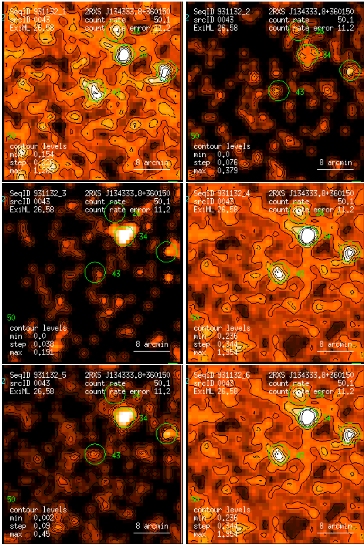
Figure 43: RASS 931132: detection 0043: band rate images, Gaussian filter: (1) PSPC channels 11 – 41, (2) 52 – 90, (3) 91 – 201, (4) 11 – 235, (5) 52 – 201, (6) 11 – 201. Broad band rates in counts/ks. Band rate contour levels in counts/ks/arcmin 2 .
