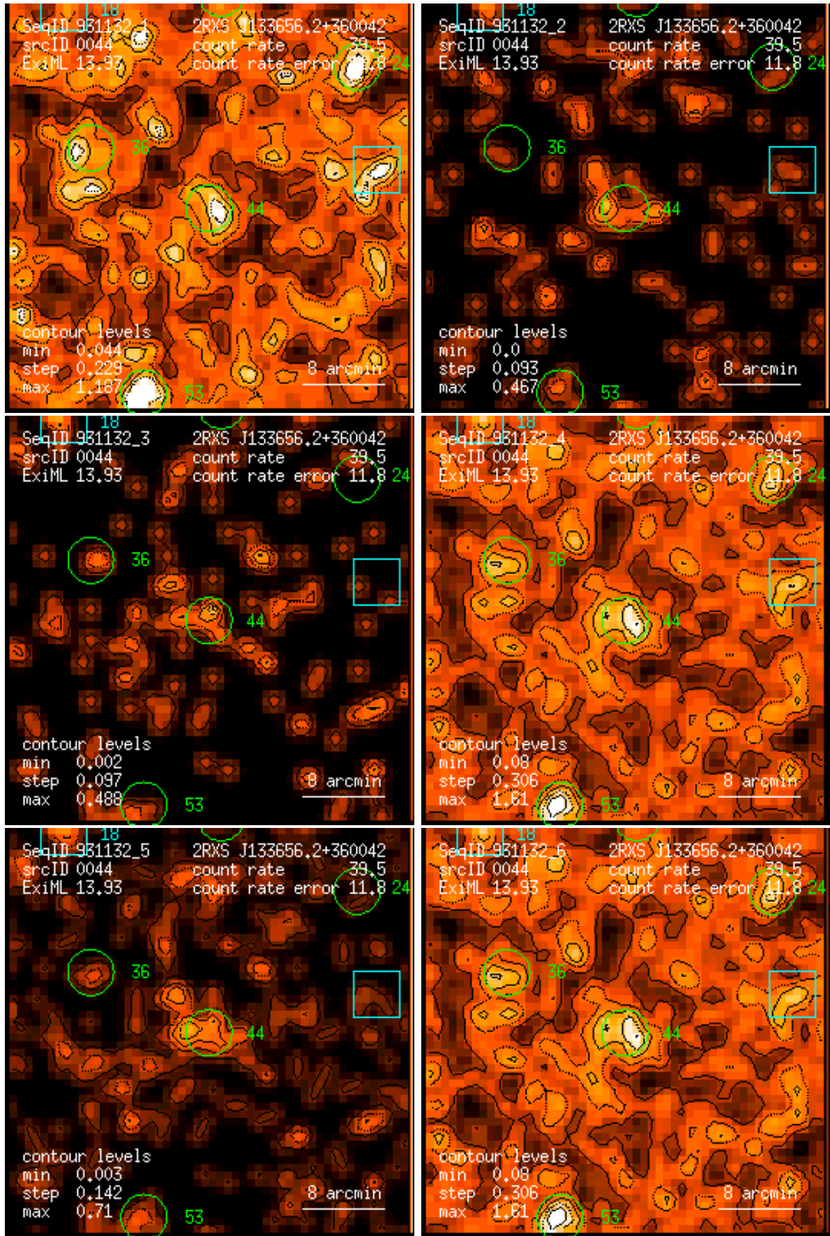
Figure 44: RASS 931132: detection 0044: band rate images, Gaussian filter: (1) PSPC channels 11 – 41, (2) 52 – 90, (3) 91 – 201, (4) 11 – 235, (5) 52 – 201, (6) 11 – 201. Broad band rates in counts/ks. Band rate contour levels in counts/ks/arcmin 2 .
