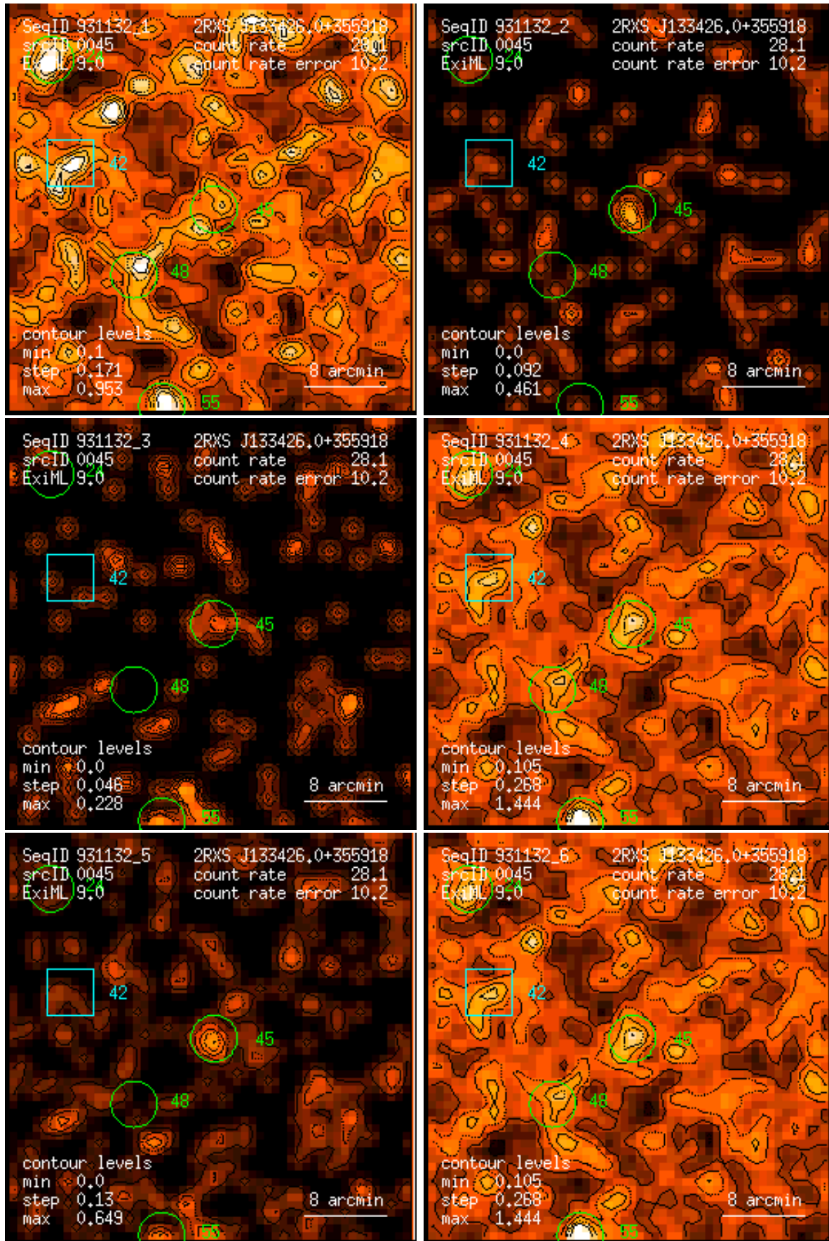
Figure 45: RASS 931132: detection 0045: band rate images, Gaussian filter: (1) PSPC channels 11 – 41, (2) 52 – 90, (3) 91 – 201, (4) 11 – 235, (5) 52 – 201, (6) 11 – 201. Broad band rates in counts/ks. Band rate contour levels in counts/ks/arcmin 2 .
