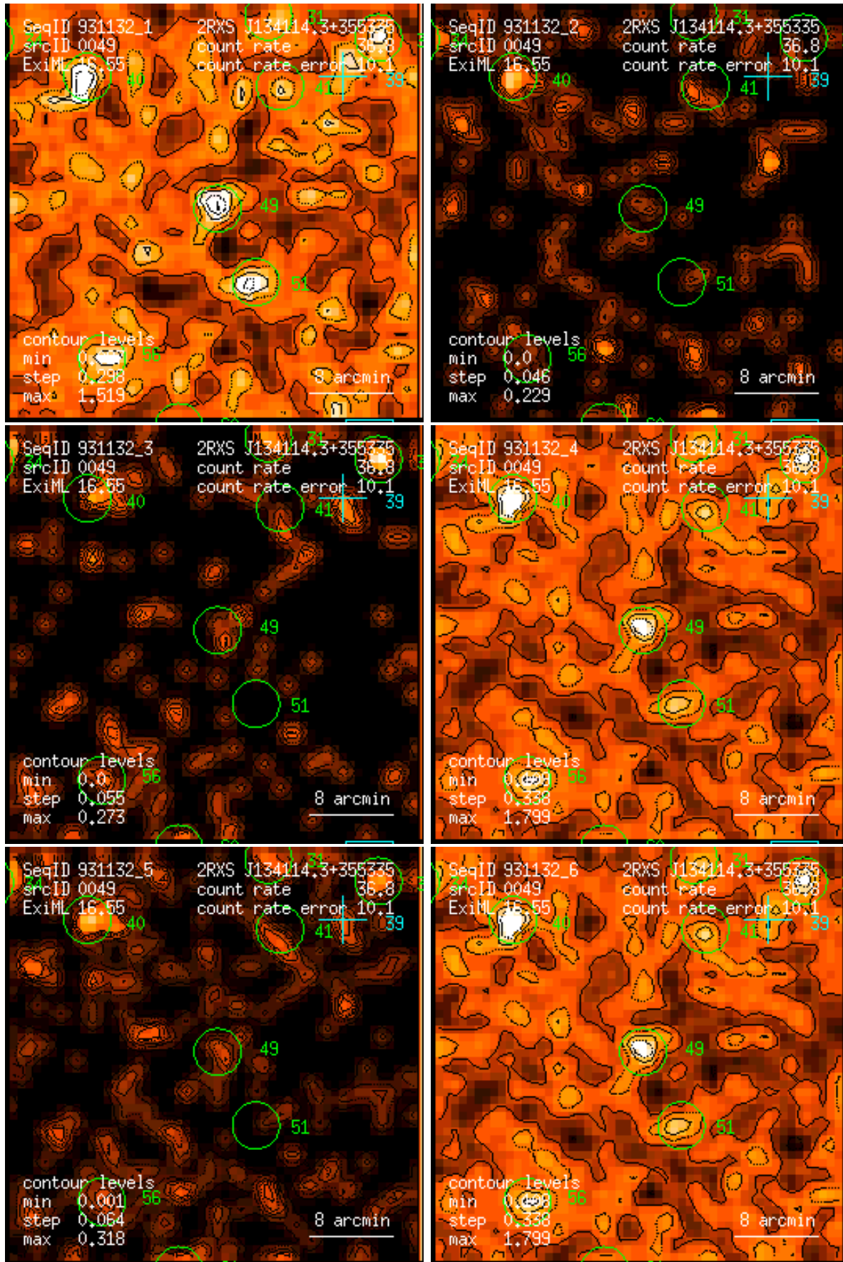
Figure 49: RASS 931132: detection 0049: band rate images, Gaussian filter: (1) PSPC channels 11 – 41, (2) 52 – 90, (3) 91 – 201, (4) 11 – 235, (5) 52 – 201, (6) 11 – 201. Broad band rates in counts/ks. Band rate contour levels in counts/ks/arcmin 2 .
