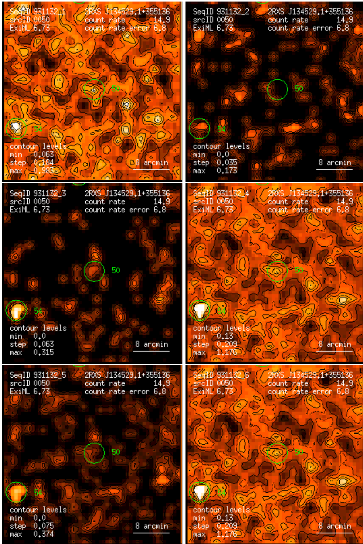
Figure 50: RASS 931132: detection 0050: band rate images, Gaussian filter: (1) PSPC channels 11 – 41, (2) 52 – 90, (3) 91 – 201, (4) 11 – 235, (5) 52 – 201, (6) 11 – 201. Broad band rates in counts/ks. Band rate contour levels in counts/ks/arcmin 2 .
