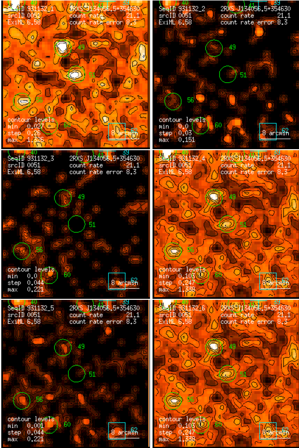
Figure 51: RASS 931132: detection 0051: band rate images, Gaussian filter: (1) PSPC channels 11 – 41, (2) 52 – 90, (3) 91 – 201, (4) 11 – 235, (5) 52 – 201, (6) 11 – 201. Broad band rates in counts/ks. Band rate contour levels in counts/ks/arcmin 2 .
