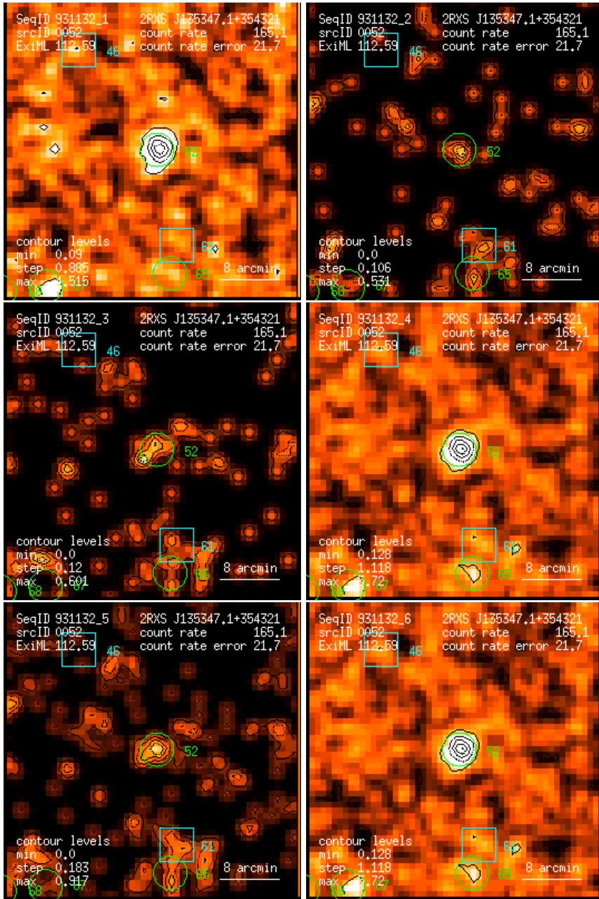
Figure 52: RASS 931132: detection 0052: band rate images, Gaussian filter: (1) PSPC channels 11 – 41, (2) 52 – 90, (3) 91 – 201, (4) 11 – 235, (5) 52 – 201, (6) 11 – 201. Broad band rates in counts/ks. Band rate contour levels in counts/ks/arcmin 2 .
