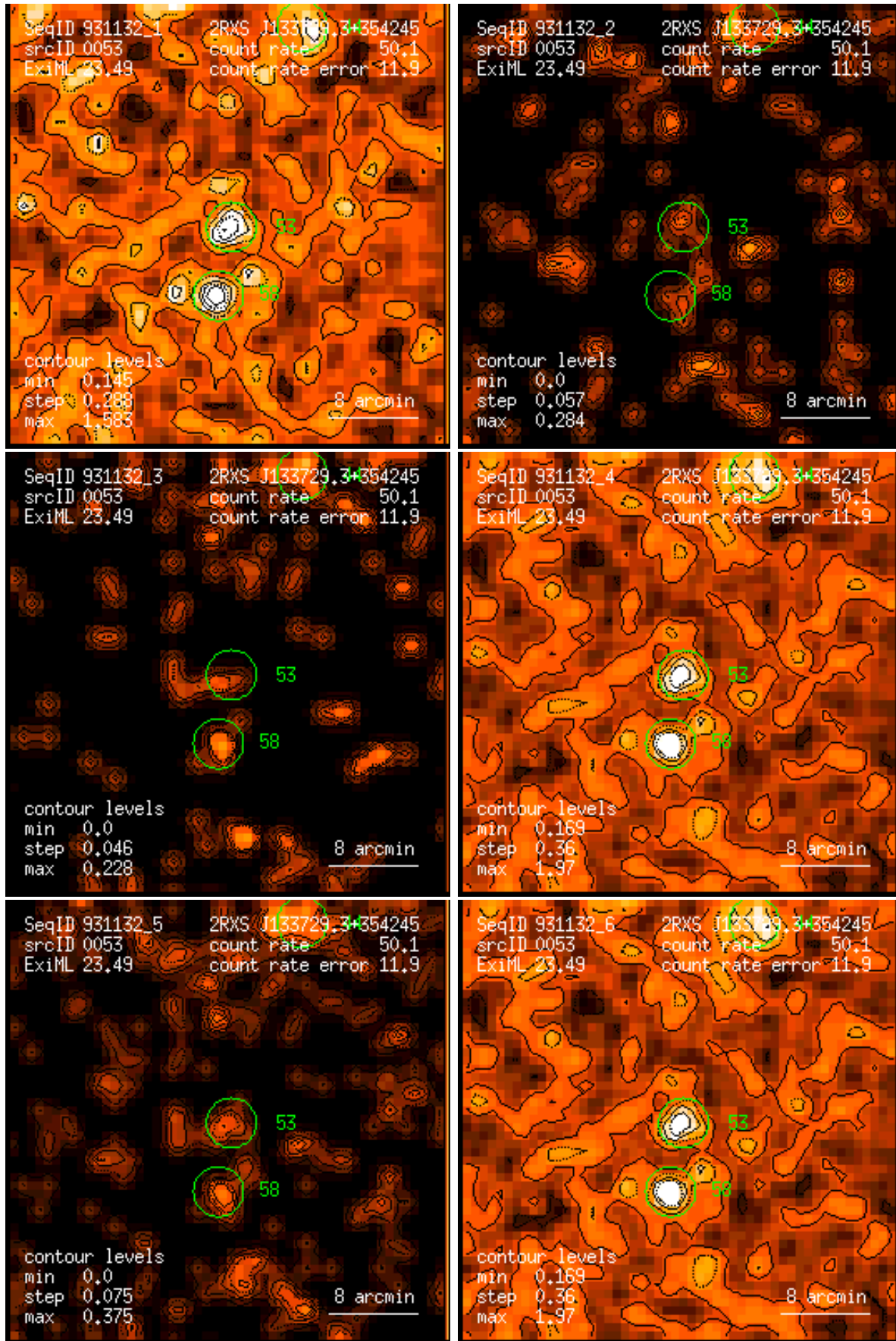
Figure 53: RASS 931132: detection 0053: band rate images, Gaussian filter: (1) PSPC channels 11 – 41, (2) 52 – 90, (3) 91 – 201, (4) 11 – 235, (5) 52 – 201, (6) 11 – 201. Broad band rates in counts/ks. Band rate contour levels in counts/ks/arcmin 2 .
