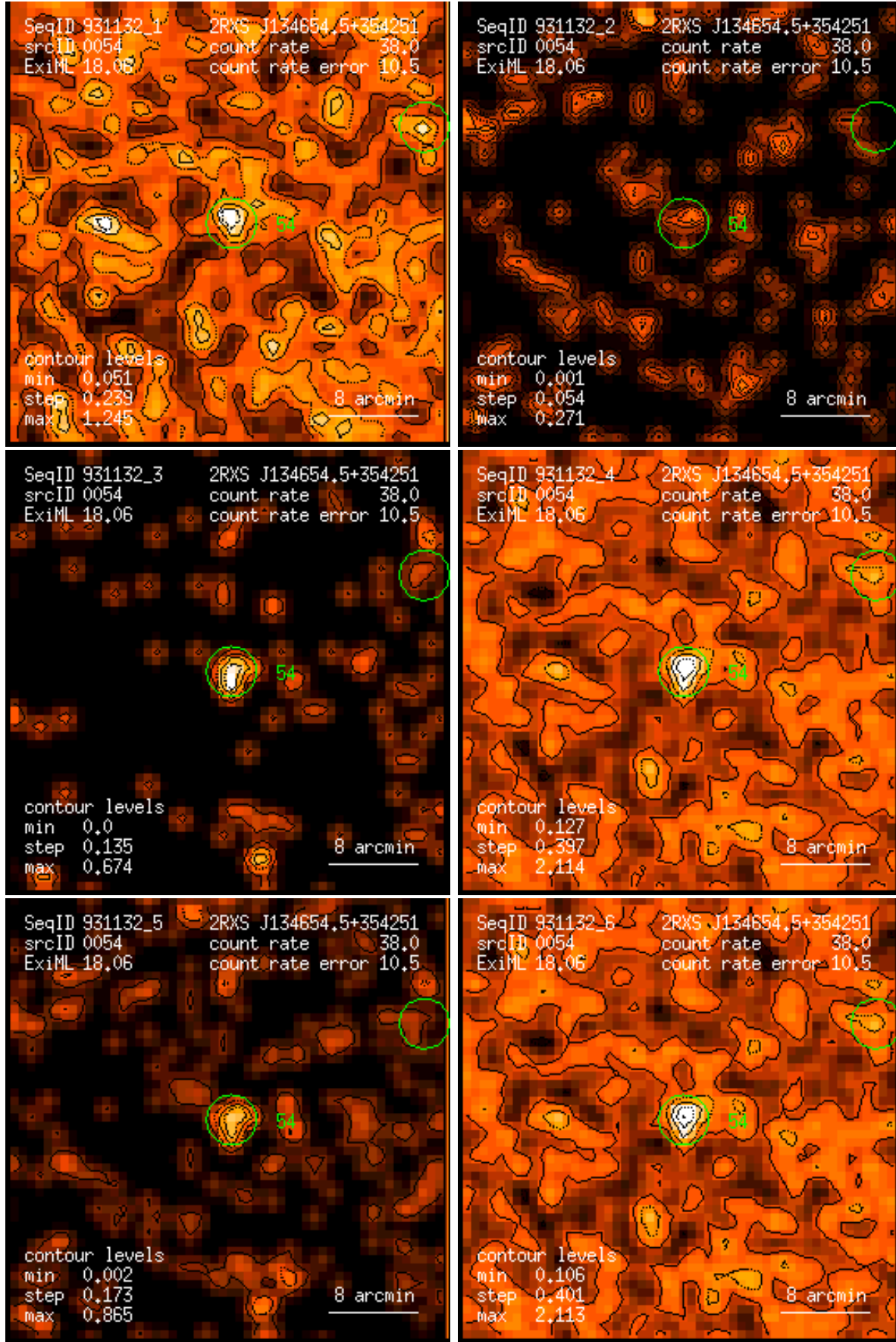
Figure 54: RASS 931132: detection 0054: band rate images, Gaussian filter: (1) PSPC channels 11 – 41, (2) 52 – 90, (3) 91 – 201, (4) 11 – 235, (5) 52 – 201, (6) 11 – 201. Broad band rates in counts/ks. Band rate contour levels in counts/ks/arcmin 2 .
