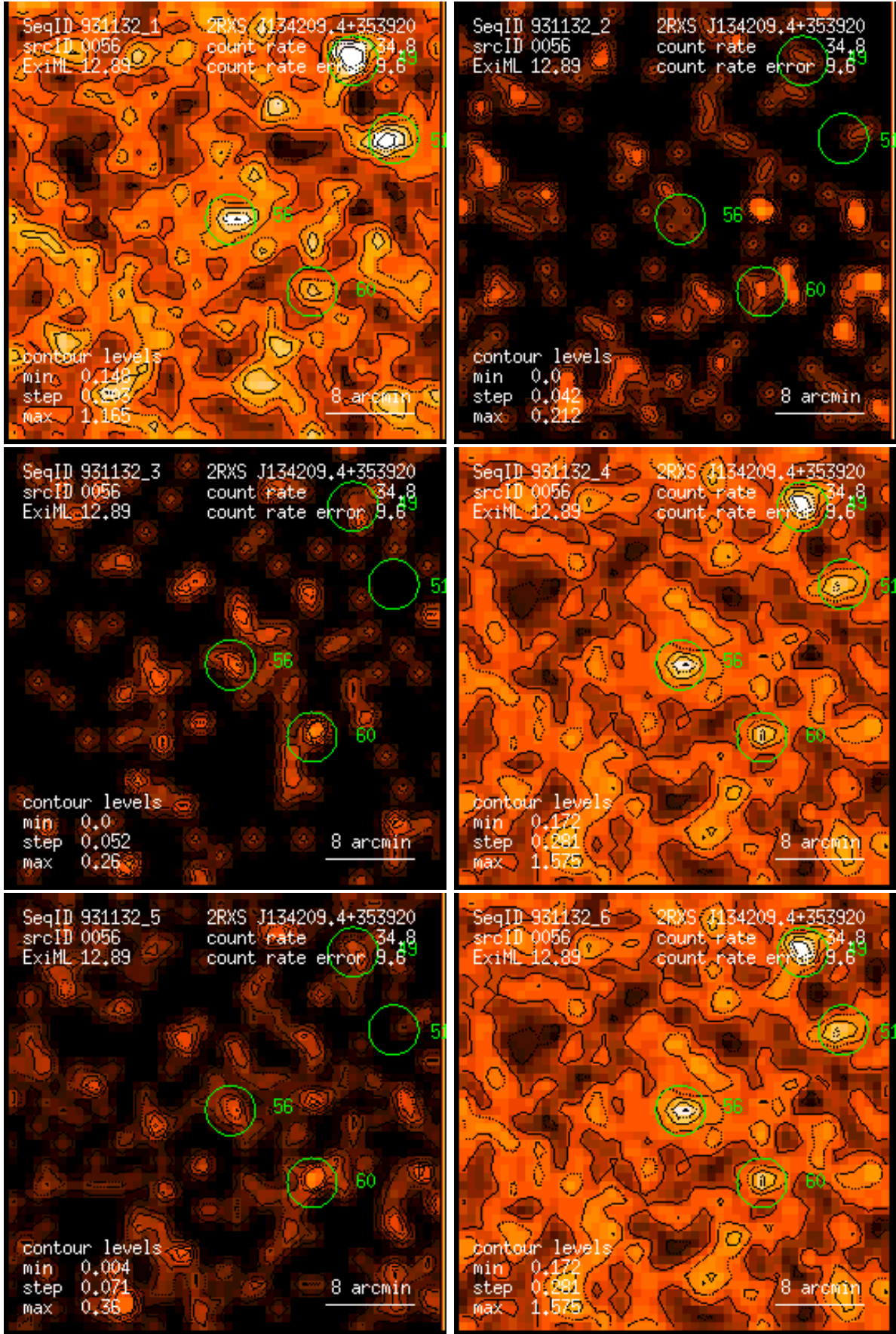
Figure 56: RASS 931132: detection 0056: band rate images, Gaussian filter: (1) PSPC channels 11 – 41, (2) 52 – 90, (3) 91 – 201, (4) 11 – 235, (5) 52 – 201, (6) 11 – 201. Broad band rates in counts/ks. Band rate contour levels in counts/ks/arcmin 2 .
