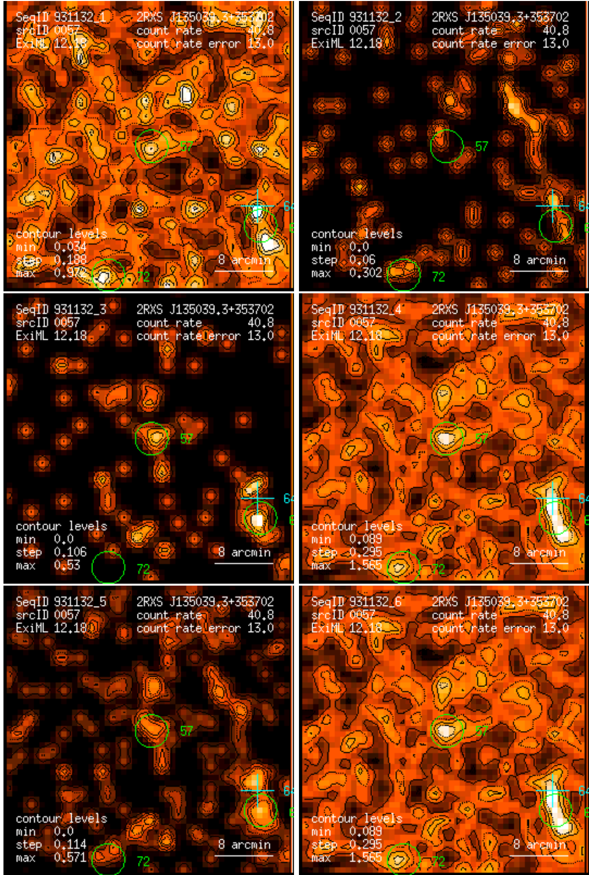
Figure 57: RASS 931132: detection 0057: band rate images, Gaussian filter: (1) PSPC channels 11 – 41, (2) 52 – 90, (3) 91 – 201, (4) 11 – 235, (5) 52 – 201, (6) 11 – 201. Broad band rates in counts/ks. Band rate contour levels in counts/ks/arcmin 2 .
