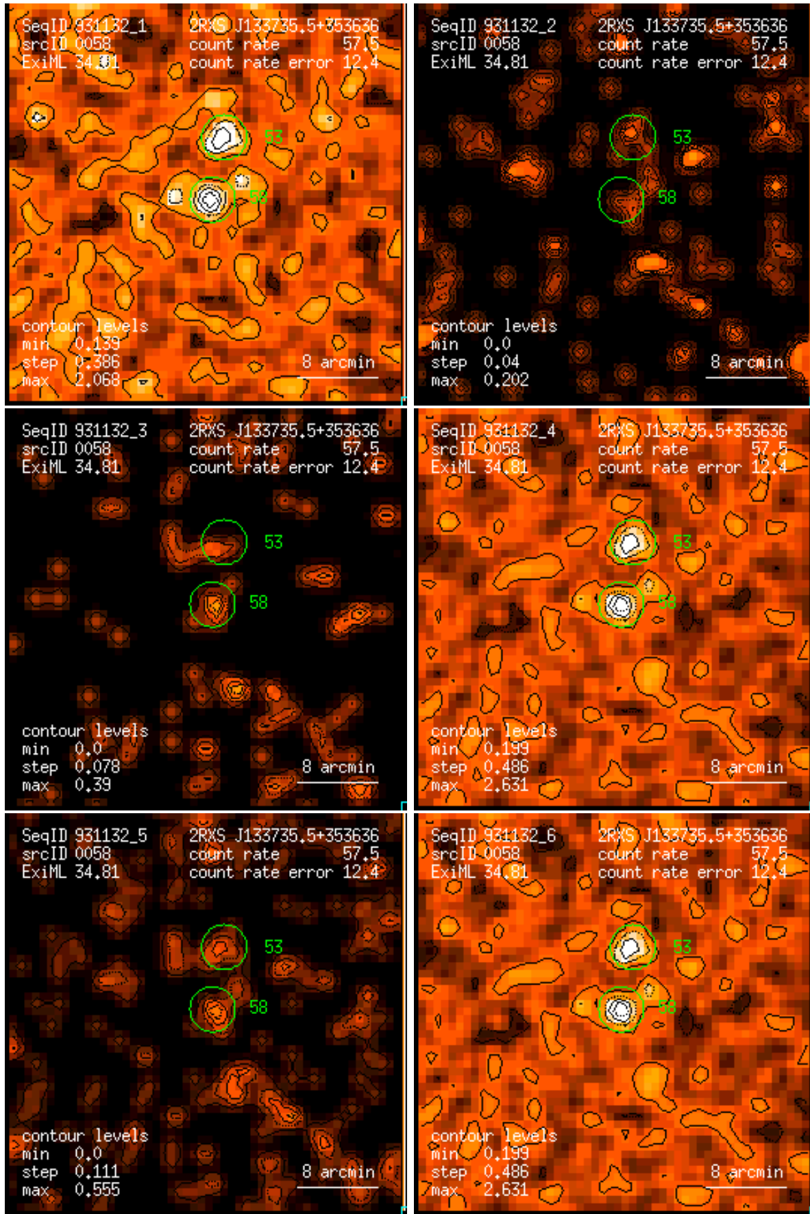
Figure 58: RASS 931132: detection 0058: band rate images, Gaussian filter: (1) PSPC channels 11 – 41, (2) 52 – 90, (3) 91 – 201, (4) 11 – 235, (5) 52 – 201, (6) 11 – 201. Broad band rates in counts/ks. Band rate contour levels in counts/ks/arcmin 2 .
