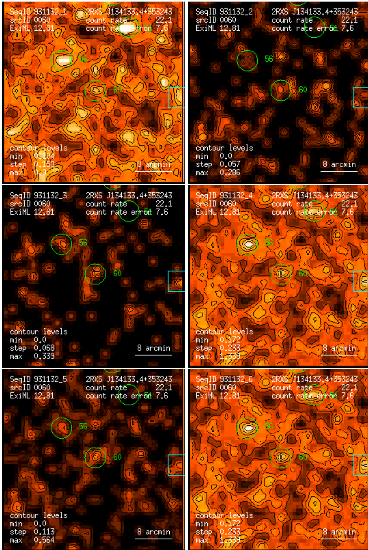
Figure 60: RASS 931132: detection 0060: band rate images, Gaussian filter: (1) PSPC channels 11 – 41, (2) 52 – 90, (3) 91 – 201, (4) 11 – 235, (5) 52 – 201, (6) 11 – 201. Broad band rates in counts/ks. Band rate contour levels in counts/ks/arcmin 2 .
