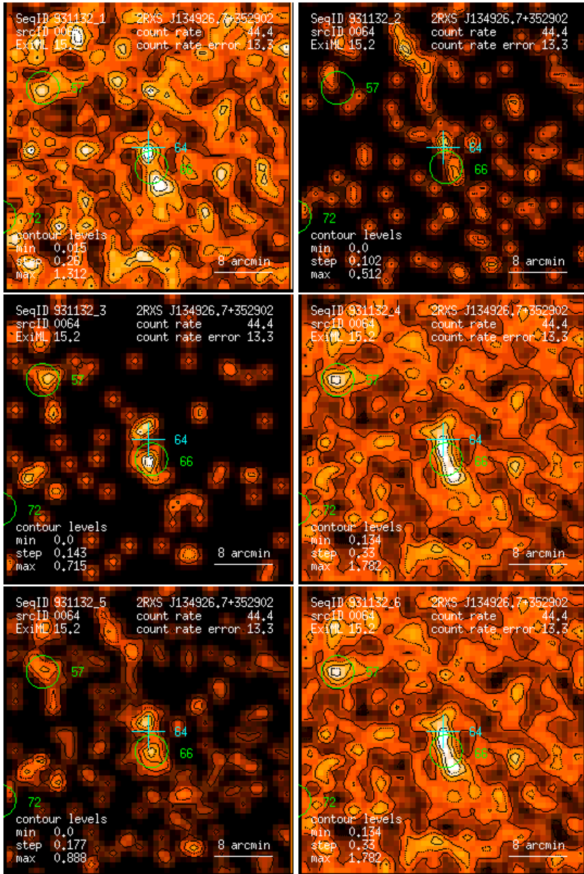
Figure 64: RASS 931132: detection 0064: band rate images, Gaussian filter: (1) PSPC channels 11 – 41, (2) 52 – 90, (3) 91 – 201, (4) 11 – 235, (5) 52 – 201, (6) 11 – 201. Broad band rates in counts/ks. Band rate contour levels in counts/ks/arcmin 2 .
