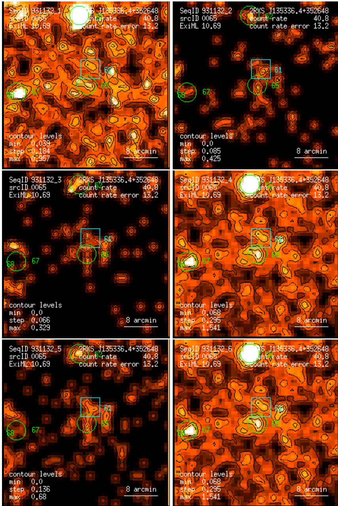
Figure 65: RASS 931132: detection 0065: band rate images, Gaussian filter: (1) PSPC channels 11 – 41, (2) 52 – 90, (3) 91 – 201, (4) 11 – 235, (5) 52 – 201, (6) 11 – 201. Broad band rates in counts/ks. Band rate contour levels in counts/ks/arcmin 2 .
