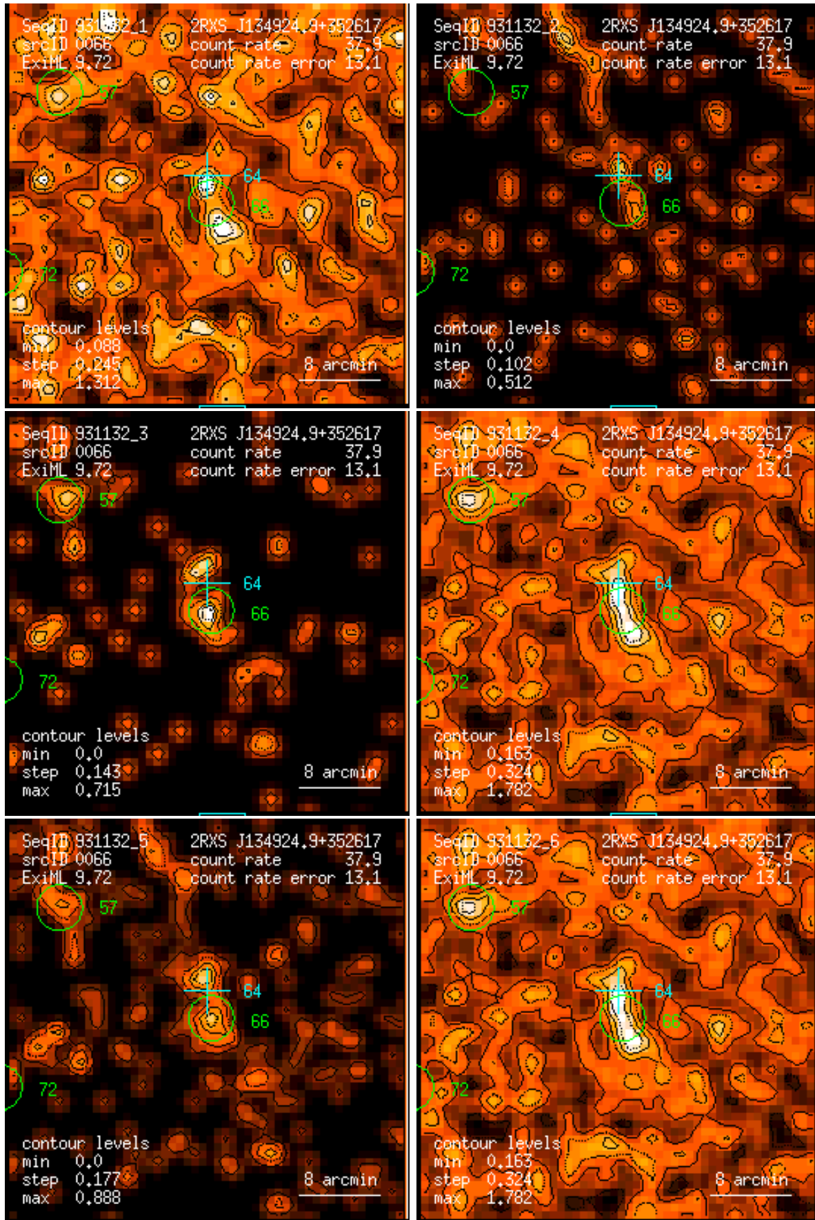
Figure 66: RASS 931132: detection 0066: band rate images, Gaussian filter: (1) PSPC channels 11 – 41, (2) 52 – 90, (3) 91 – 201, (4) 11 – 235, (5) 52 – 201, (6) 11 – 201. Broad band rates in counts/ks. Band rate contour levels in counts/ks/arcmin 2 .
