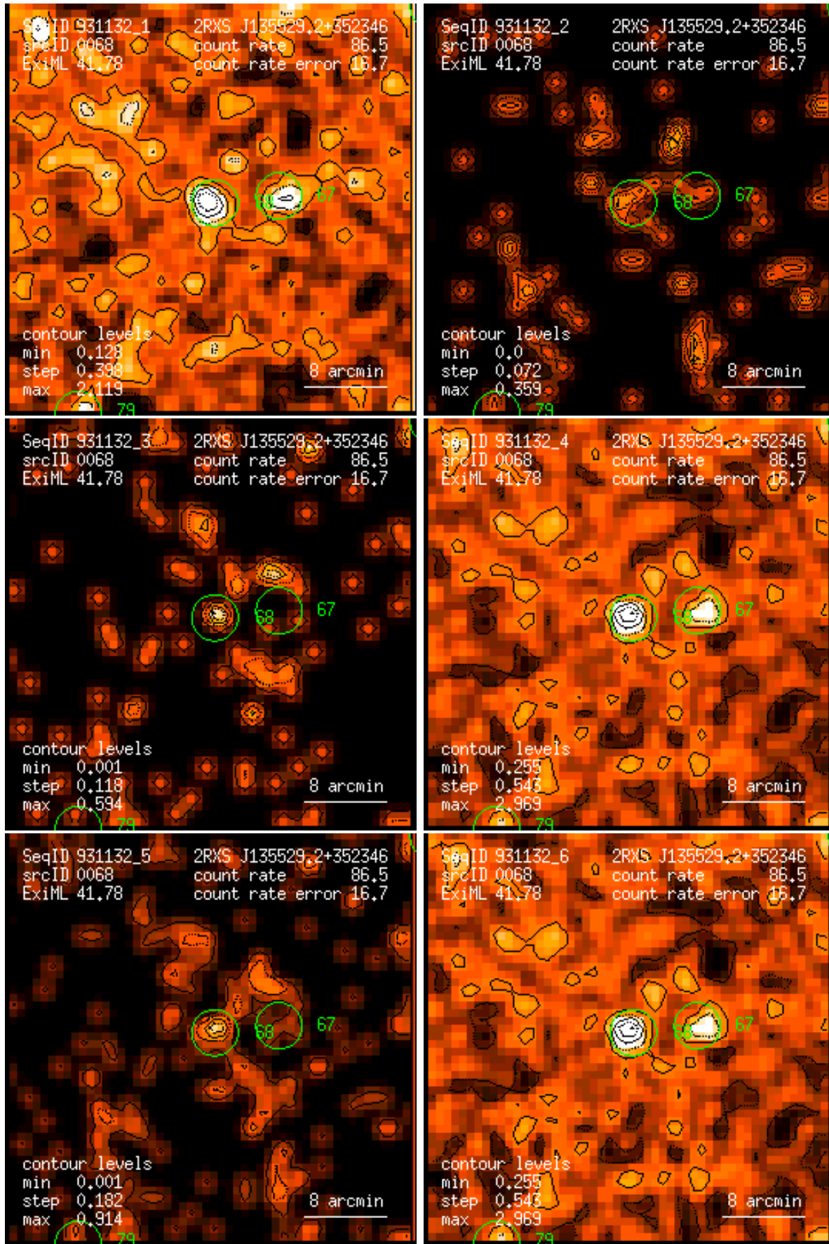
Figure 68: RASS 931132: detection 0068: band rate images, Gaussian filter: (1) PSPC channels 11 – 41, (2) 52 – 90, (3) 91 – 201, (4) 11 – 235, (5) 52 – 201, (6) 11 – 201. Broad band rates in counts/ks. Band rate contour levels in counts/ks/arcmin 2 .
