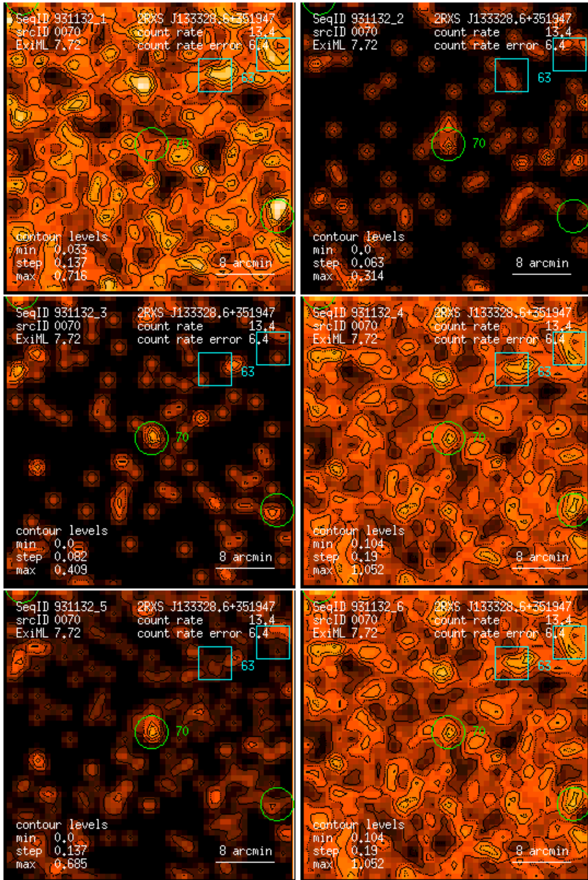
Figure 70: RASS 931132: detection 0070: band rate images, Gaussian filter: (1) PSPC channels 11 – 41, (2) 52 – 90, (3) 91 – 201, (4) 11 – 235, (5) 52 – 201, (6) 11 – 201. Broad band rates in counts/ks. Band rate contour levels in counts/ks/arcmin 2 .
