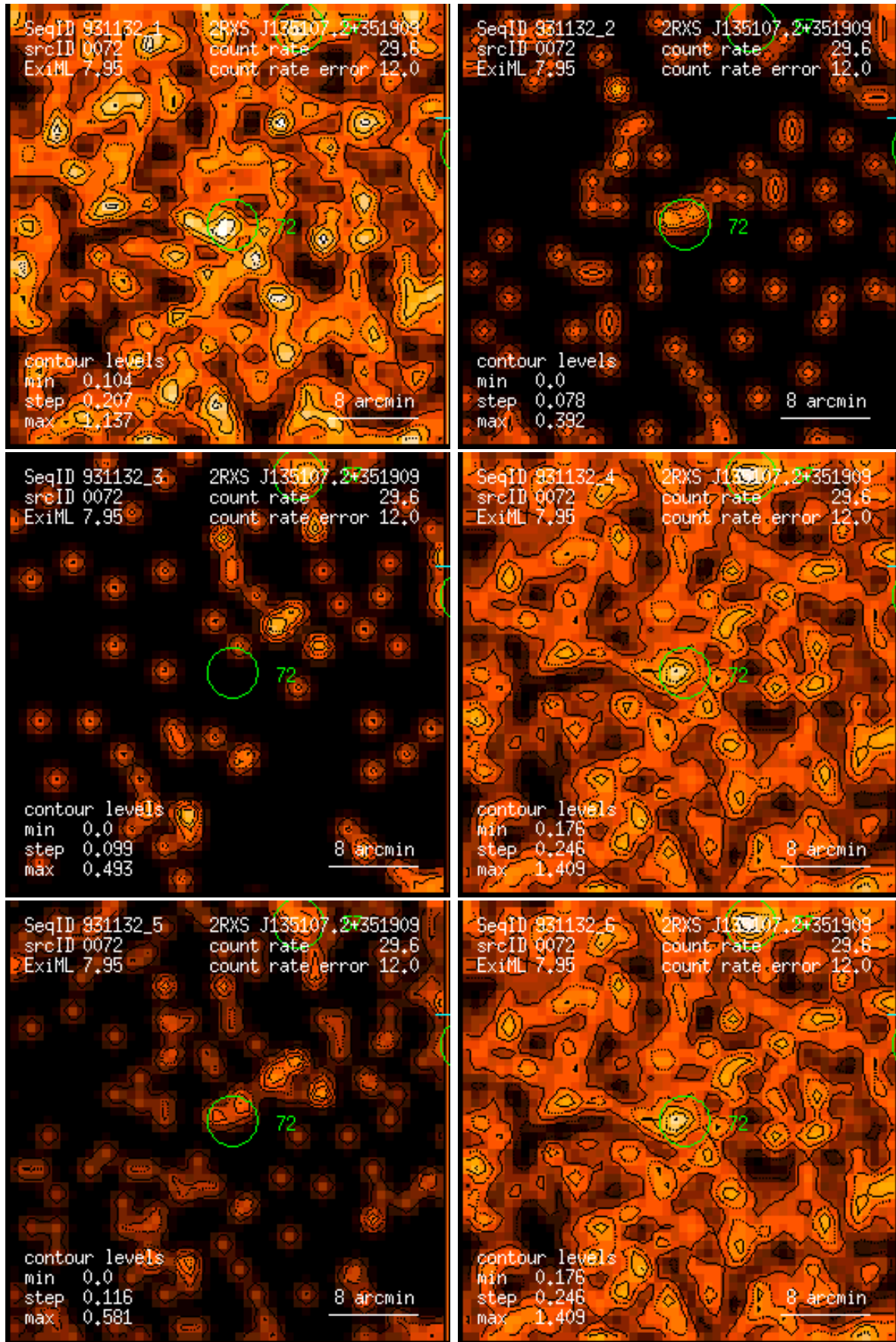
Figure 72: RASS 931132: detection 0072: band rate images, Gaussian filter: (1) PSPC channels 11 – 41, (2) 52 – 90, (3) 91 – 201, (4) 11 – 235, (5) 52 – 201, (6) 11 – 201. Broad band rates in counts/ks. Band rate contour levels in counts/ks/arcmin 2 .
