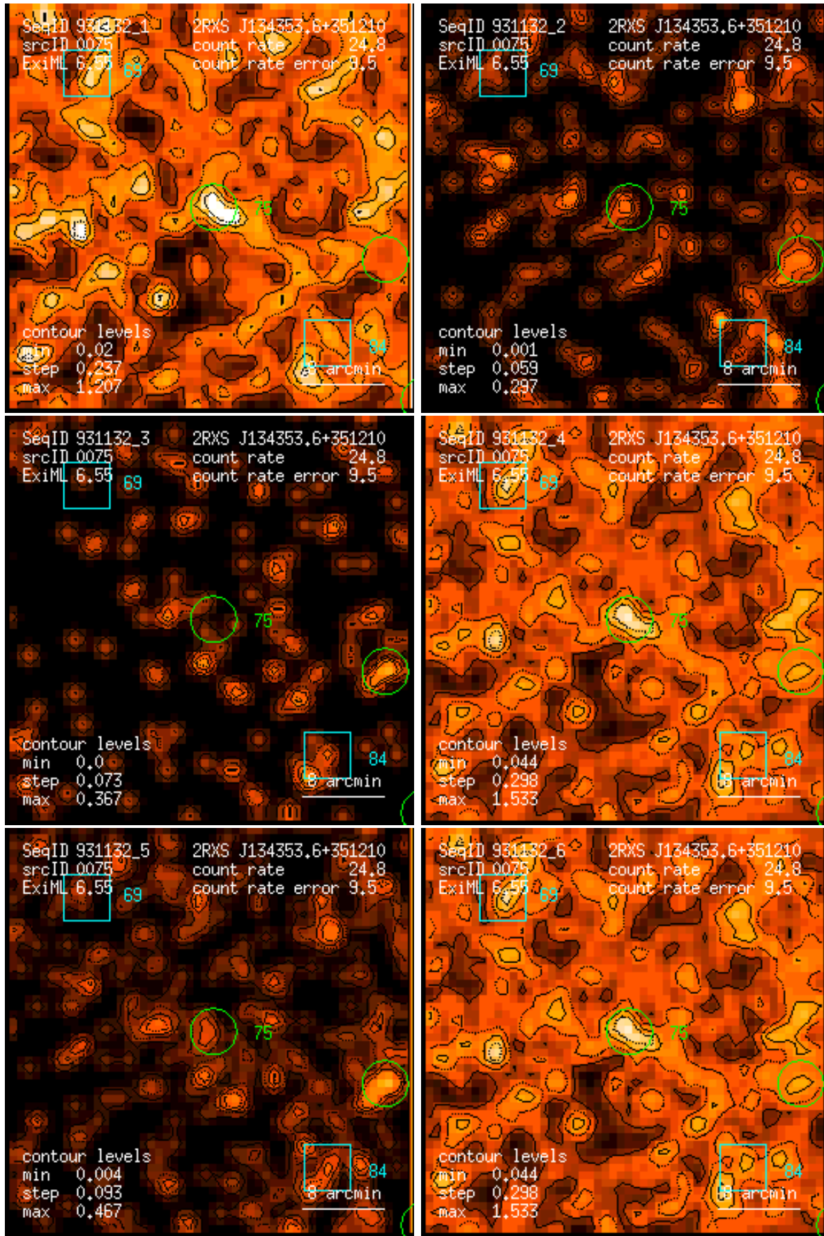
Figure 75: RASS 931132: detection 0075: band rate images, Gaussian filter: (1) PSPC channels 11 – 41, (2) 52 – 90, (3) 91 – 201, (4) 11 – 235, (5) 52 – 201, (6) 11 – 201. Broad band rates in counts/ks. Band rate contour levels in counts/ks/arcmin 2 .
