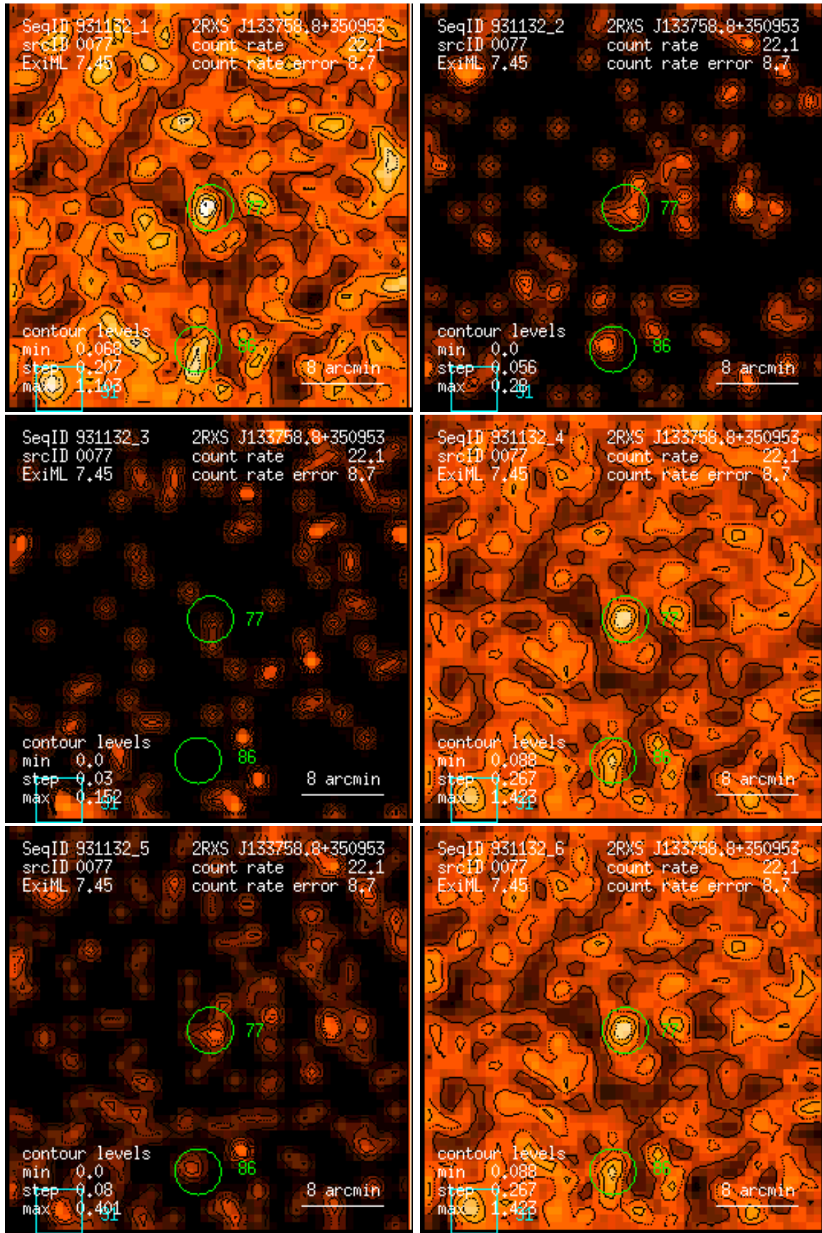
Figure 77: RASS 931132: detection 0077: band rate images, Gaussian filter: (1) PSPC channels 11 – 41, (2) 52 – 90, (3) 91 – 201, (4) 11 – 235, (5) 52 – 201, (6) 11 – 201. Broad band rates in counts/ks. Band rate contour levels in counts/ks/arcmin 2 .
