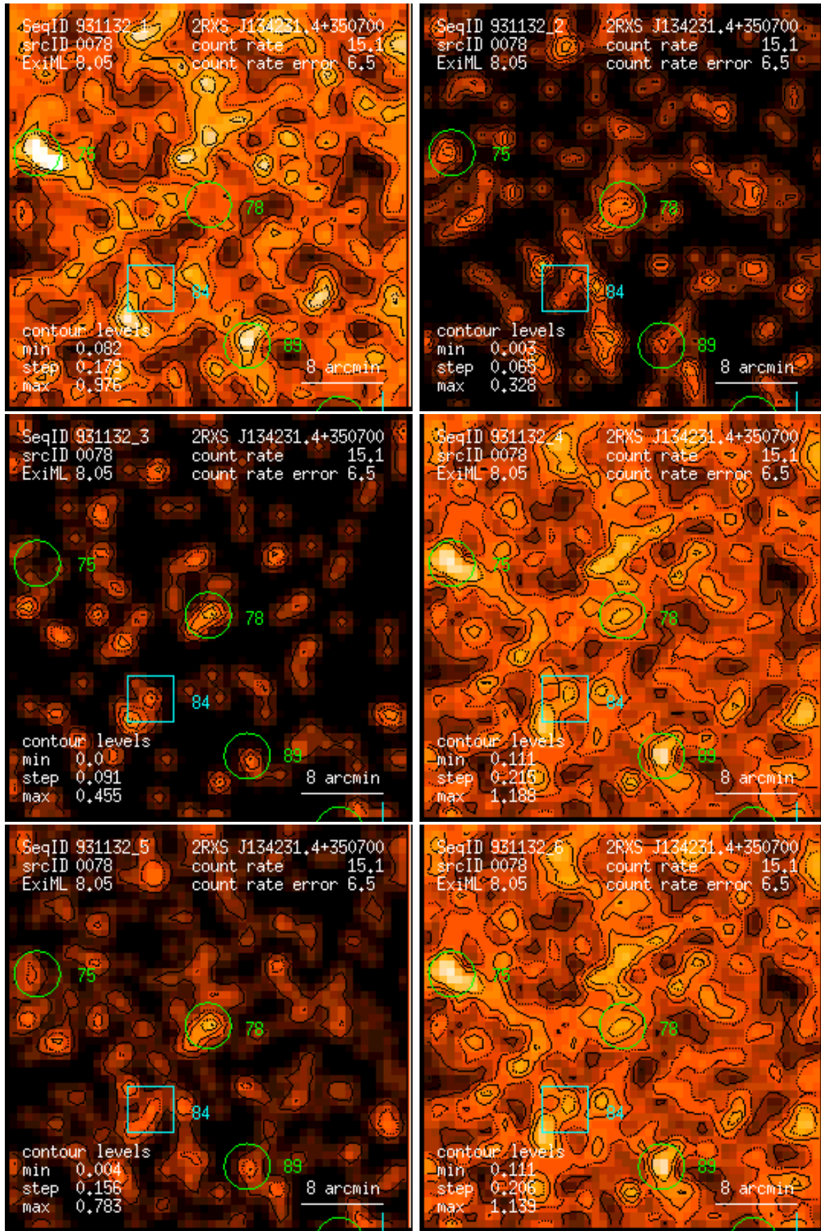
Figure 78: RASS 931132: detection 0078: band rate images, Gaussian filter: (1) PSPC channels 11 – 41, (2) 52 – 90, (3) 91 – 201, (4) 11 – 235, (5) 52 – 201, (6) 11 – 201. Broad band rates in counts/ks. Band rate contour levels in counts/ks/arcmin 2 .
