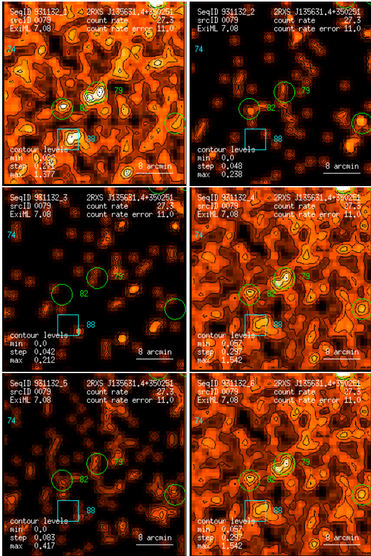
Figure 79: RASS 931132: detection 0079: band rate images, Gaussian filter: (1) PSPC channels 11 – 41, (2) 52 – 90, (3) 91 – 201, (4) 11 – 235, (5) 52 – 201, (6) 11 – 201. Broad band rates in counts/ks. Band rate contour levels in counts/ks/arcmin 2 .
