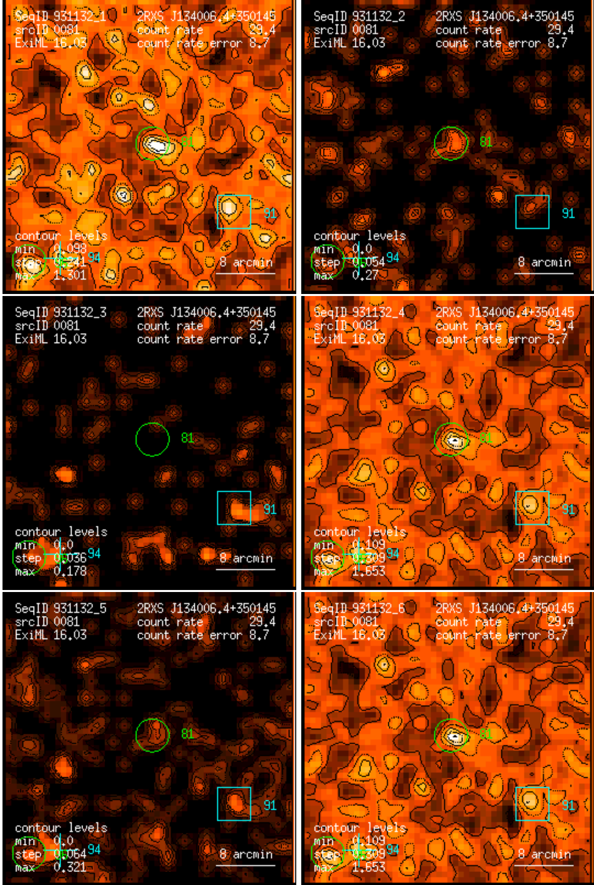
Figure 81: RASS 931132: detection 0081: band rate images, Gaussian filter: (1) PSPC channels 11 – 41, (2) 52 – 90, (3) 91 – 201, (4) 11 – 235, (5) 52 – 201, (6) 11 – 201. Broad band rates in counts/ks. Band rate contour levels in counts/ks/arcmin 2 .
