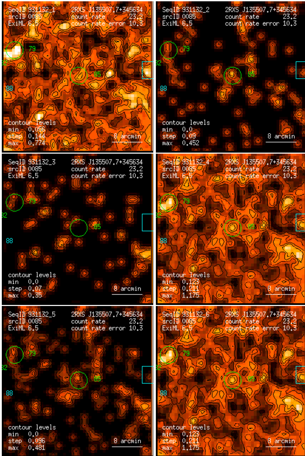
Figure 85: RASS 931132: detection 0085: band rate images, Gaussian filter: (1) PSPC channels 11 – 41, (2) 52 – 90, (3) 91 – 201, (4) 11 – 235, (5) 52 – 201, (6) 11 – 201. Broad band rates in counts/ks. Band rate contour levels in counts/ks/arcmin 2 .
