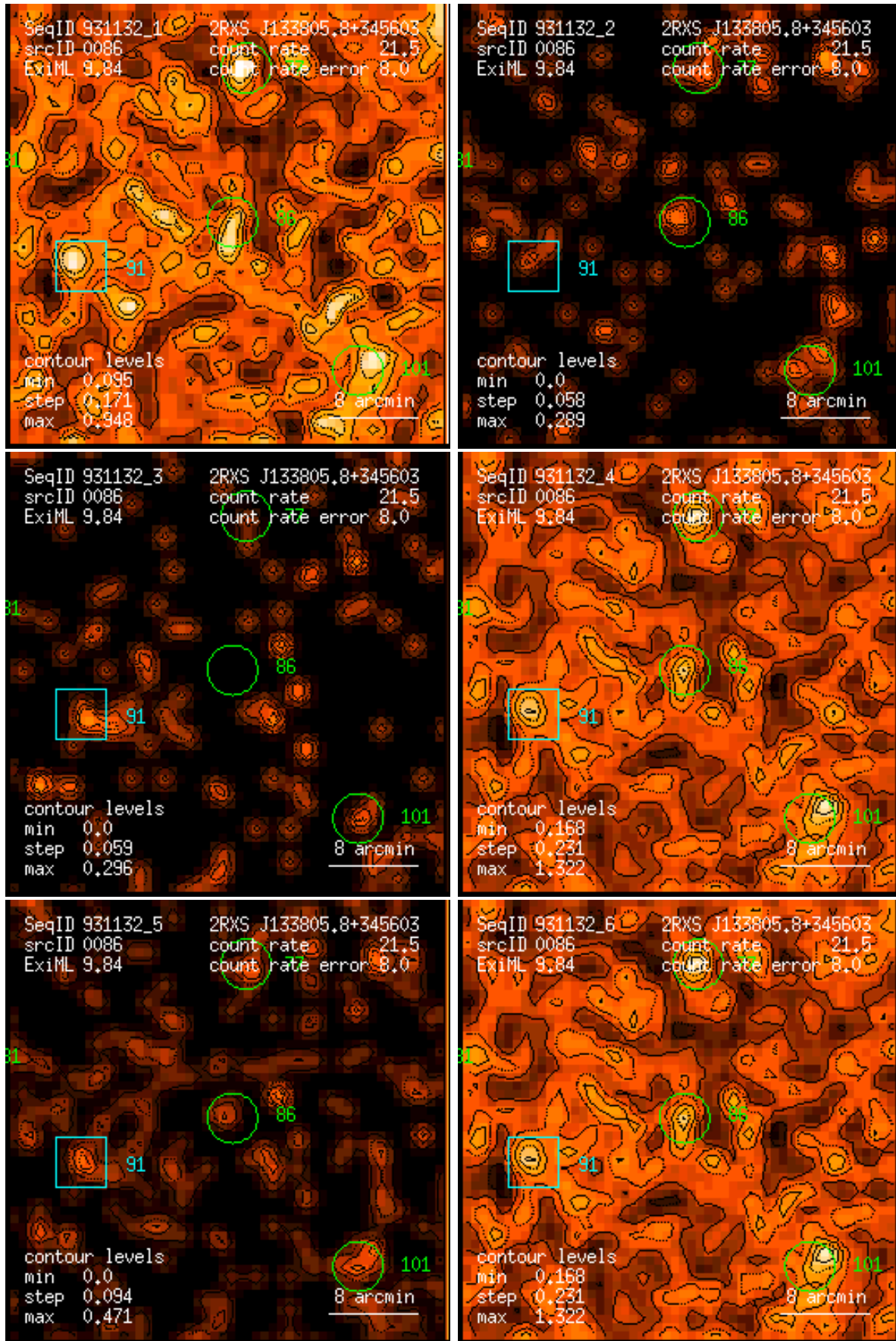
Figure 86: RASS 931132: detection 0086: band rate images, Gaussian filter: (1) PSPC channels 11 – 41, (2) 52 – 90, (3) 91 – 201, (4) 11 – 235, (5) 52 – 201, (6) 11 – 201. Broad band rates in counts/ks. Band rate contour levels in counts/ks/arcmin 2 .
