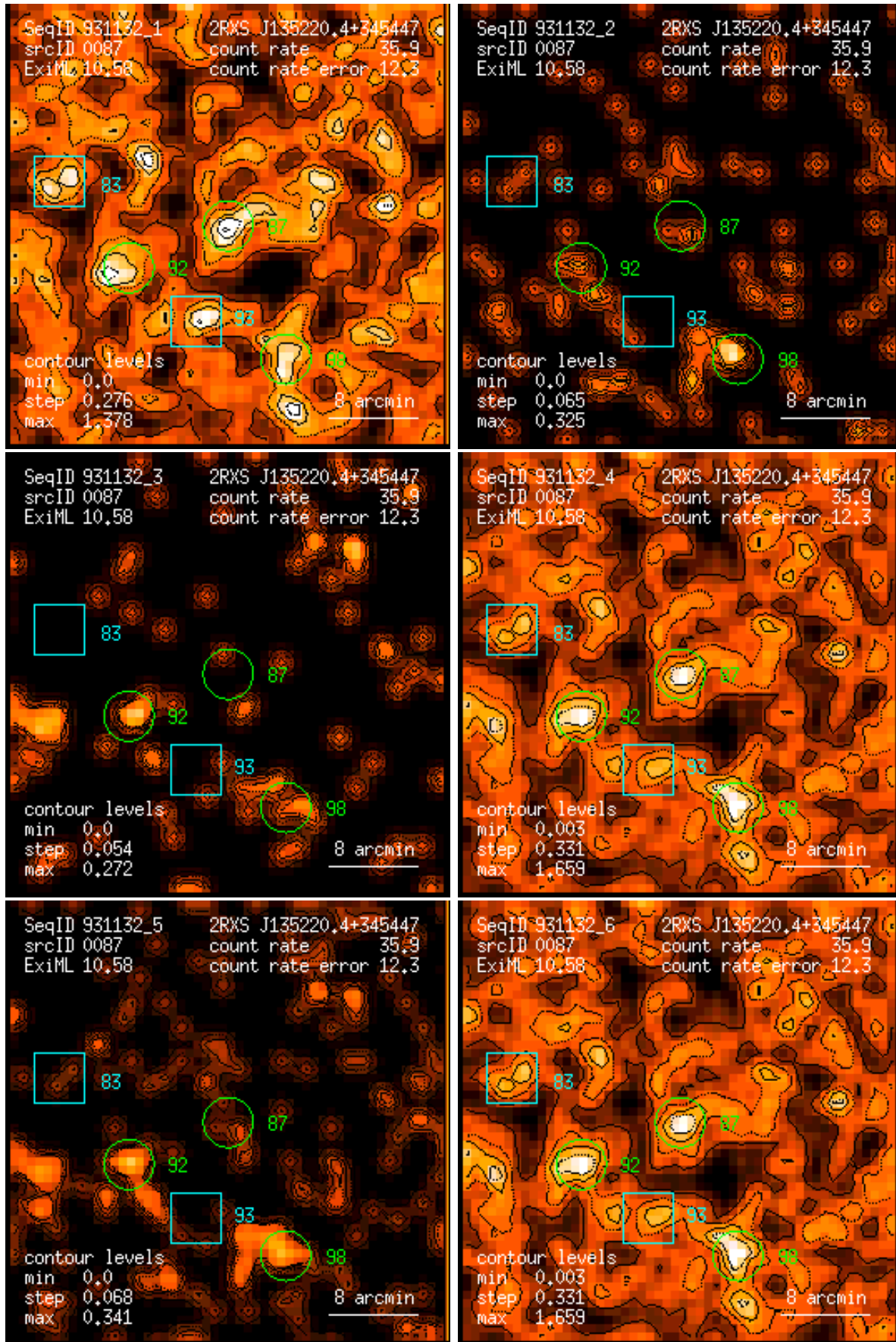
Figure 87: RASS 931132: detection 0087: band rate images, Gaussian filter: (1) PSPC channels 11 – 41, (2) 52 – 90, (3) 91 – 201, (4) 11 – 235, (5) 52 – 201, (6) 11 – 201. Broad band rates in counts/ks. Band rate contour levels in counts/ks/arcmin 2 .
