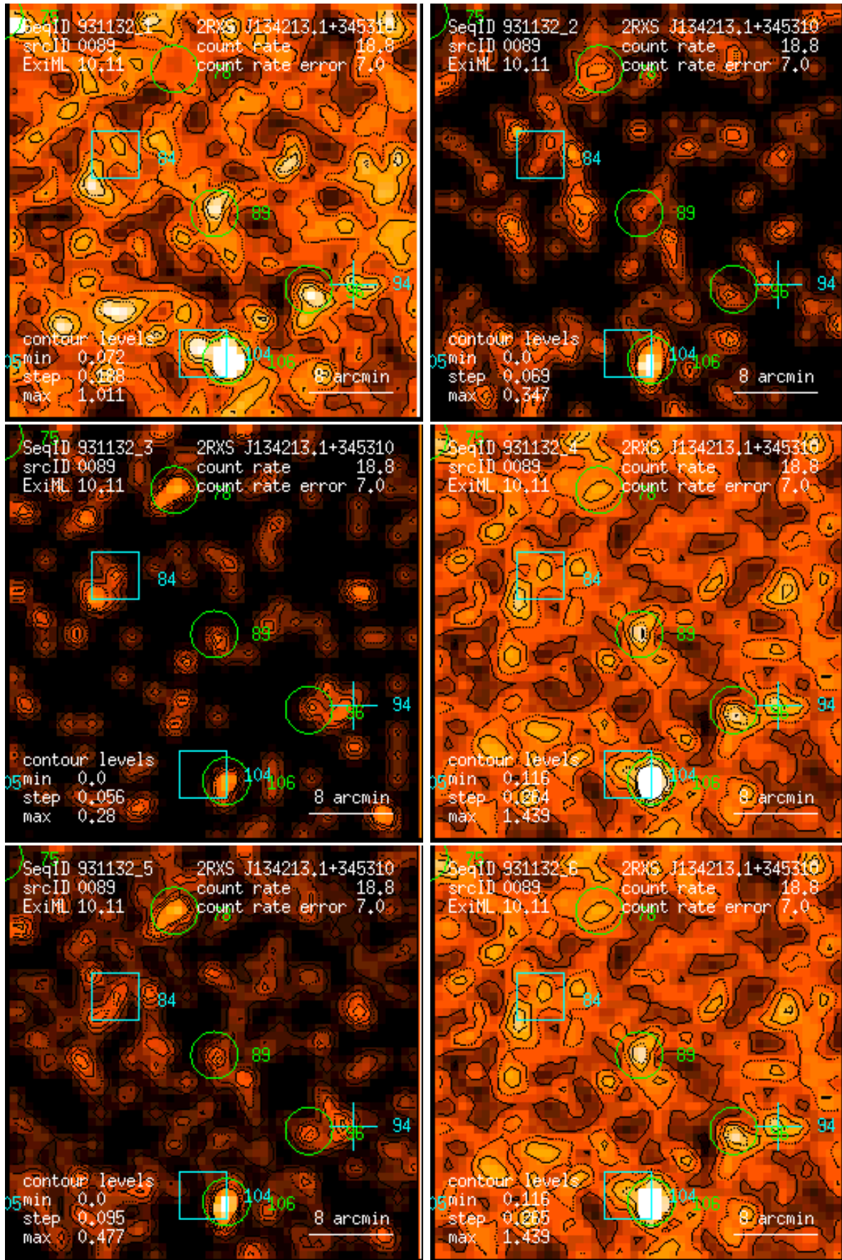
Figure 89: RASS 931132: detection 0089: band rate images, Gaussian filter: (1) PSPC channels 11 – 41, (2) 52 – 90, (3) 91 – 201, (4) 11 – 235, (5) 52 – 201, (6) 11 – 201. Broad band rates in counts/ks. Band rate contour levels in counts/ks/arcmin 2 .
