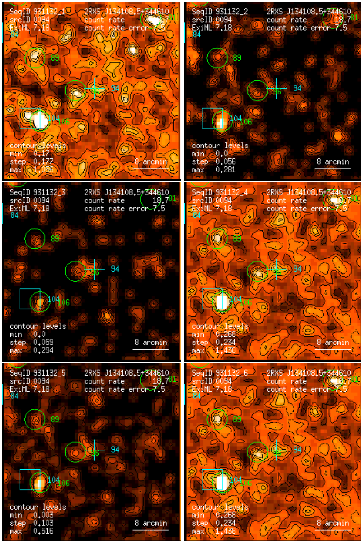
Figure 94: RASS 931132: detection 0094: band rate images, Gaussian filter: (1) PSPC channels 11 – 41, (2) 52 – 90, (3) 91 – 201, (4) 11 – 235, (5) 52 – 201, (6) 11 – 201. Broad band rates in counts/ks. Band rate contour levels in counts/ks/arcmin 2 .
