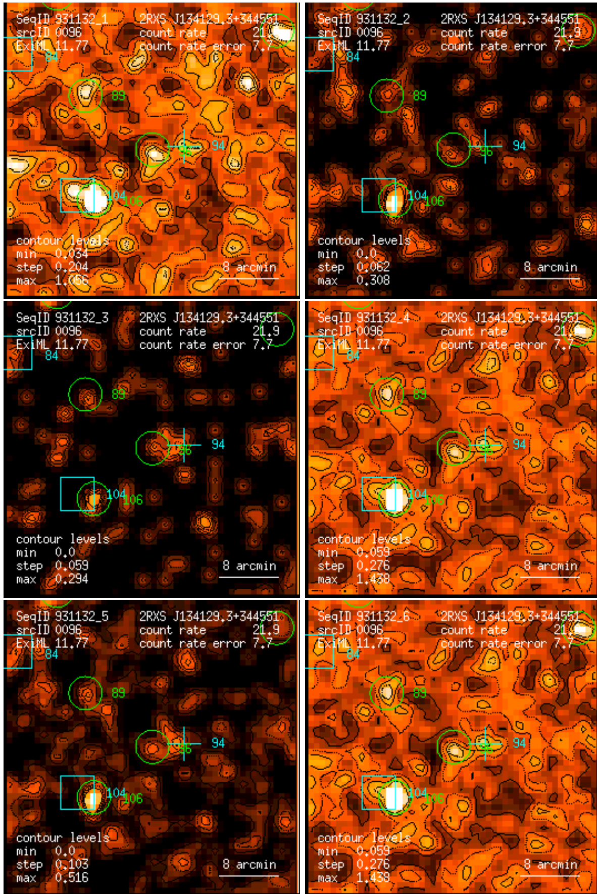
Figure 96: RASS 931132: detection 0096: band rate images, Gaussian filter: (1) PSPC channels 11 – 41, (2) 52 – 90, (3) 91 – 201, (4) 11 – 235, (5) 52 – 201, (6) 11 – 201. Broad band rates in counts/ks. Band rate contour levels in counts/ks/arcmin 2 .
